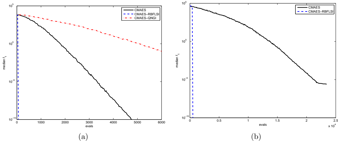
Figure 3. Convergence graphs for, f_1 , the Schewefel 1.2 quadratic, unimodal function in 10 (a) and 30 (b) dimensions. Convergence is nearly instantaneous for CMAES-RBFLSI once enough points are obtained for an interpolant.
