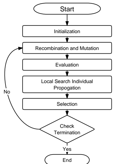
Figure 2. Flowchart for the hybrid evolution strategy algorithm
