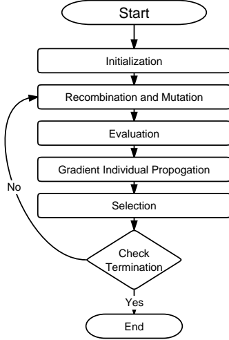
Figure 1: Flowchart for the hybrid evolution strategy algorithm
