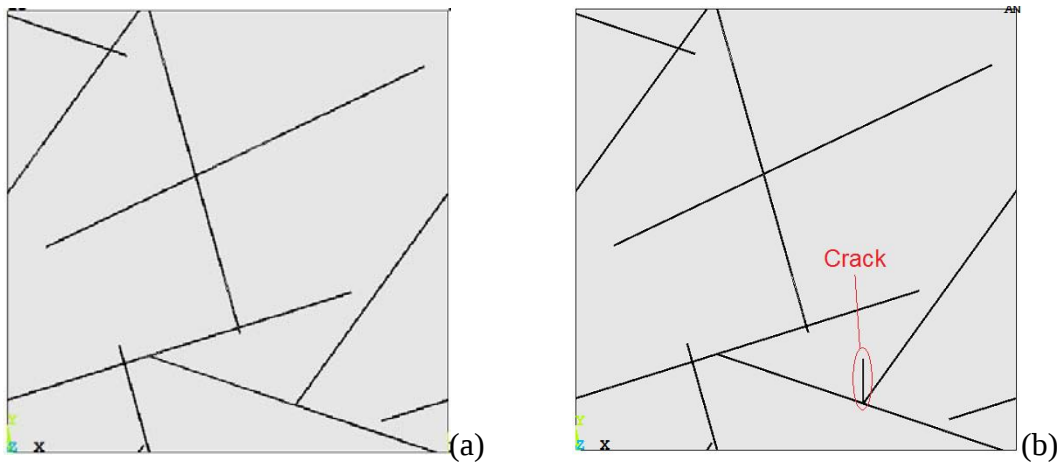
Figure 6. 2D FE model of composite layer: (a) healthy structure, (b) damaged with a crack
