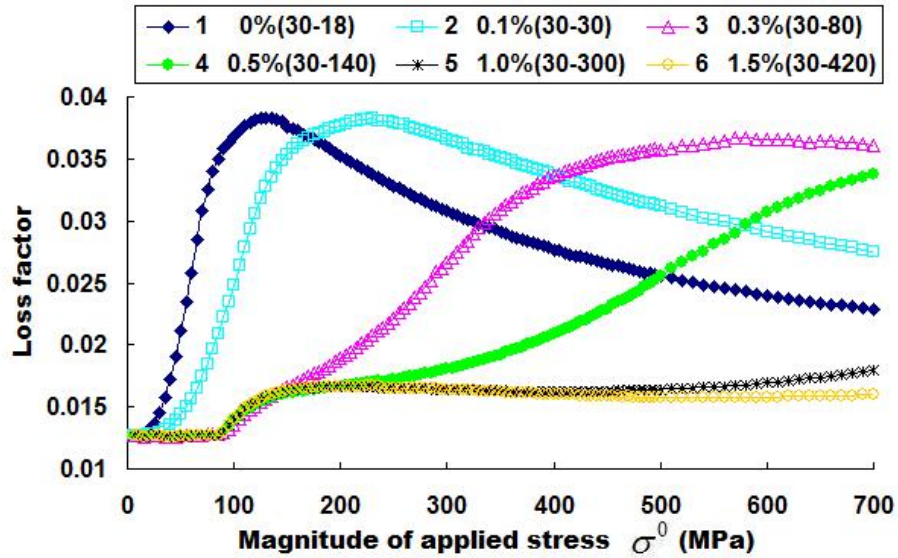
Figure 2. Loss factor of epoxy composite with in-plane randomly-oriented functionalized SWNT ropes under tension-compression cyclic loading. The legend indicates the case number, the CNT functionalization scale, and the corresponding two interfacial shear strengths at the inter-tube and CNT/epoxy interface. For instance, 1 0% (30-18) represents Case 1 for a composite with non-functionalized CNTs, which has inter-tube shear strength of 30 MPa and CNT/epoxy shear strength of 18 MPa.
