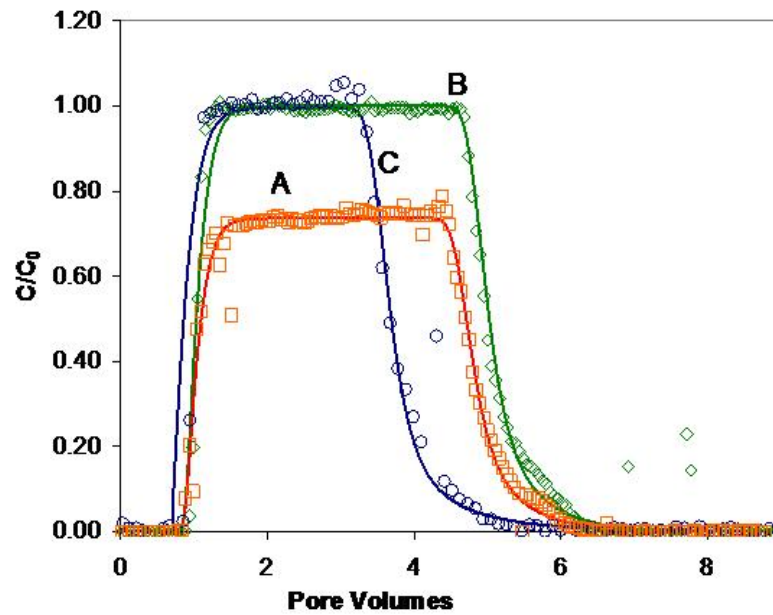
Figure III-51. Simulation of emulsion transport in federal fine sand using a modified filtration model.
