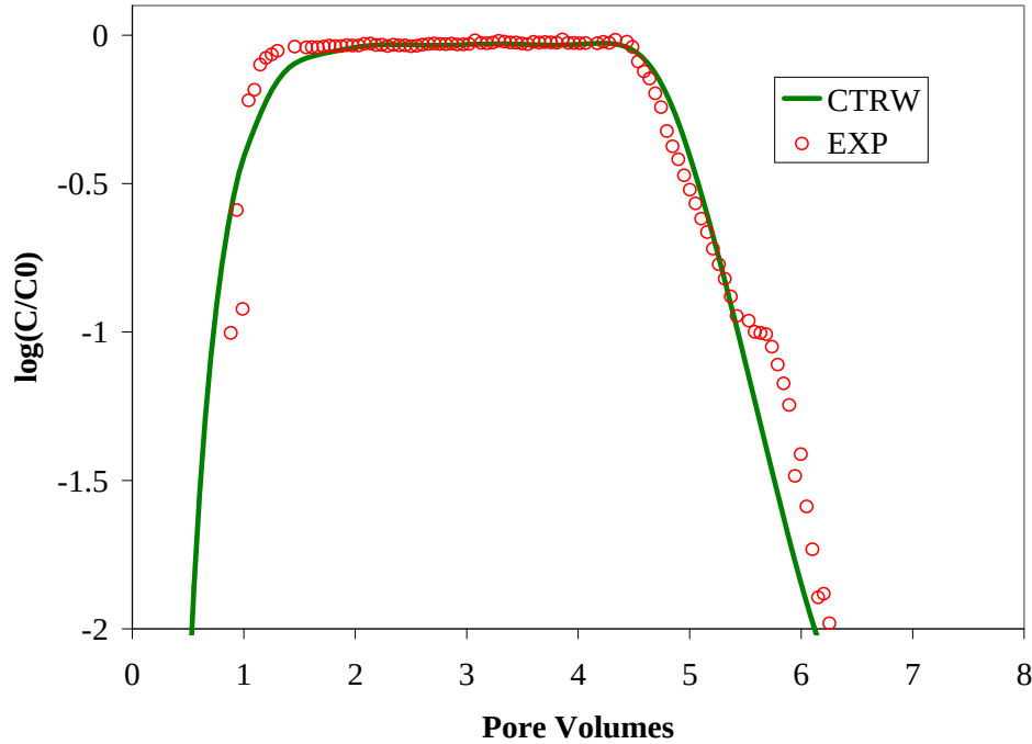
Figure III-49. Simulation of emulsion A transport in Federal Fine sand using Continuous Time Random Walk.
