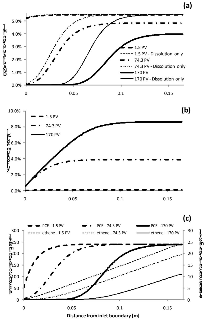
Figure III-56. Spatial distribution profiles of (a) DNAPL saturation, (b) \text{Fe}^0 content of soil, and (c) dissolved PCE and ethene concentrations at different simulation times.
