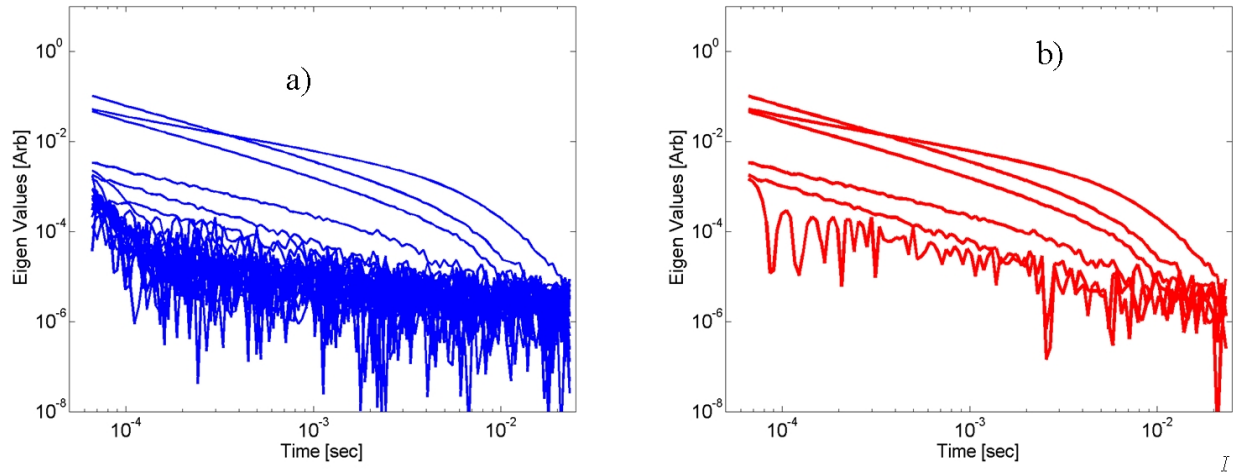
Figure 12: Eigenvalues versus time for 4.2'' mortar TEMENTADS data: a) All 25 eigenvalues. b) The three highest eigenvalues are associated with the 4.2'' mortar and the next three correspond to non dipole terms.
