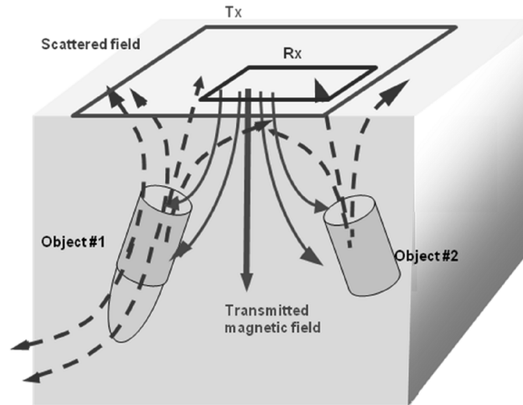
Figure 10: Metallic objects under the transmitter. The target's EMI response at the receiver coil can be calculated from the volume magnetic dipole moment d\mathbf{m} .
