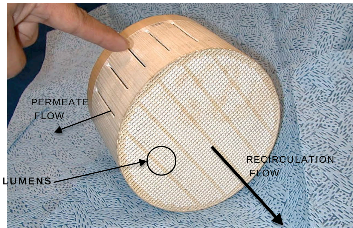
Figure 2. Ceramic Membrane Element (a short piece)
