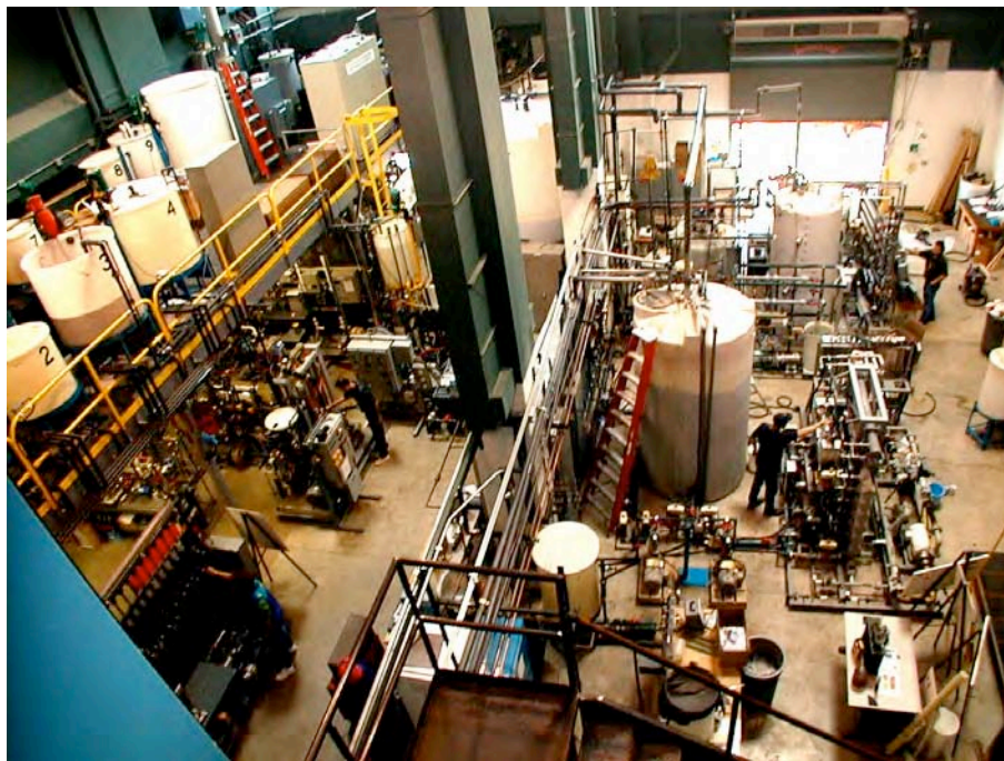
Figure 7 - Liquid waste laboratory at NSWCCD
