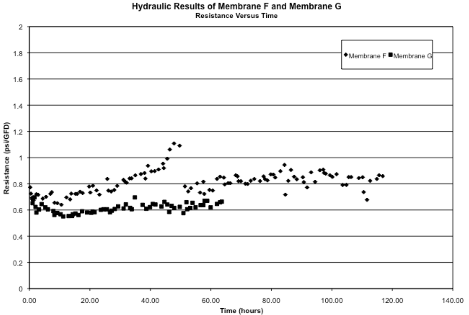
Figure 11. Resistance curves of Membranes F and G, both of which passed.
