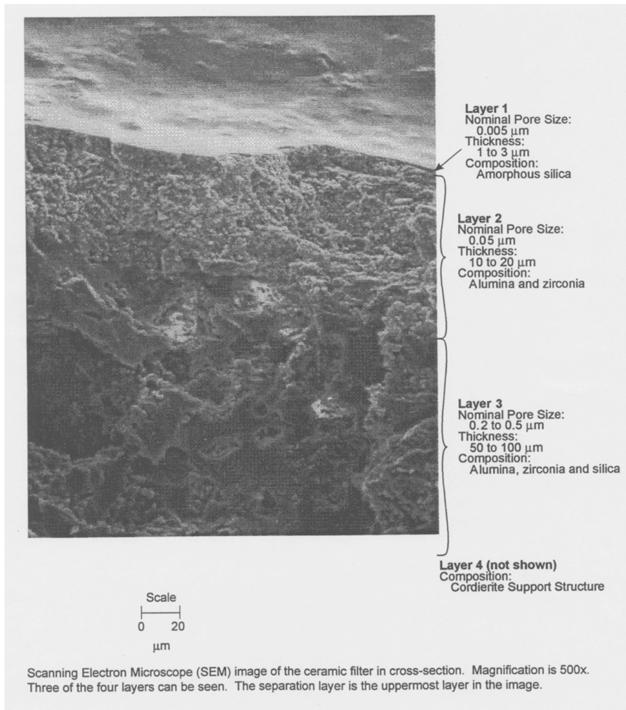
Figure 4. Ceramic membrane layers without the non-porous polymer coating.
