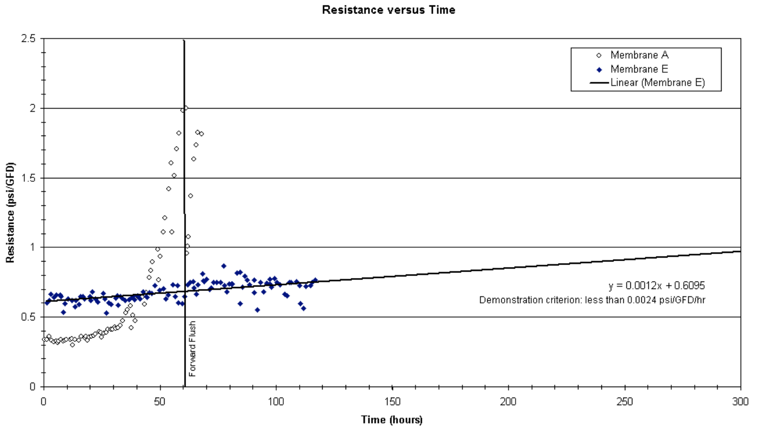
Figure 10. Graph of resistance versus time for uncoated (A) and coated (E) membranes.
