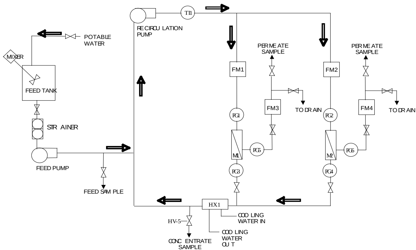
Figure 8. Schematic of the membrane test loop
