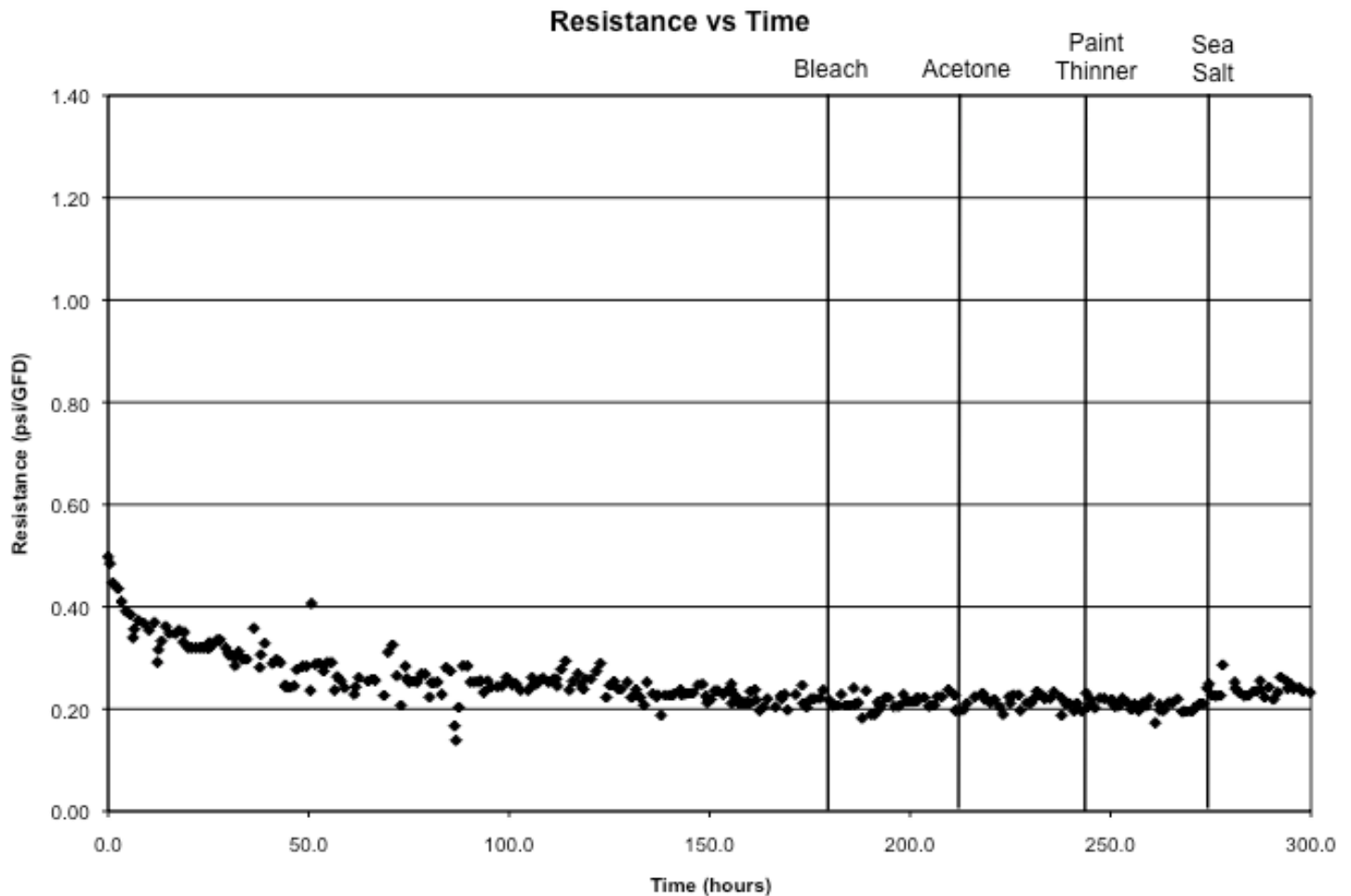
Figure 17. Chemical stability tests of full-scale membrane with polymer coating
