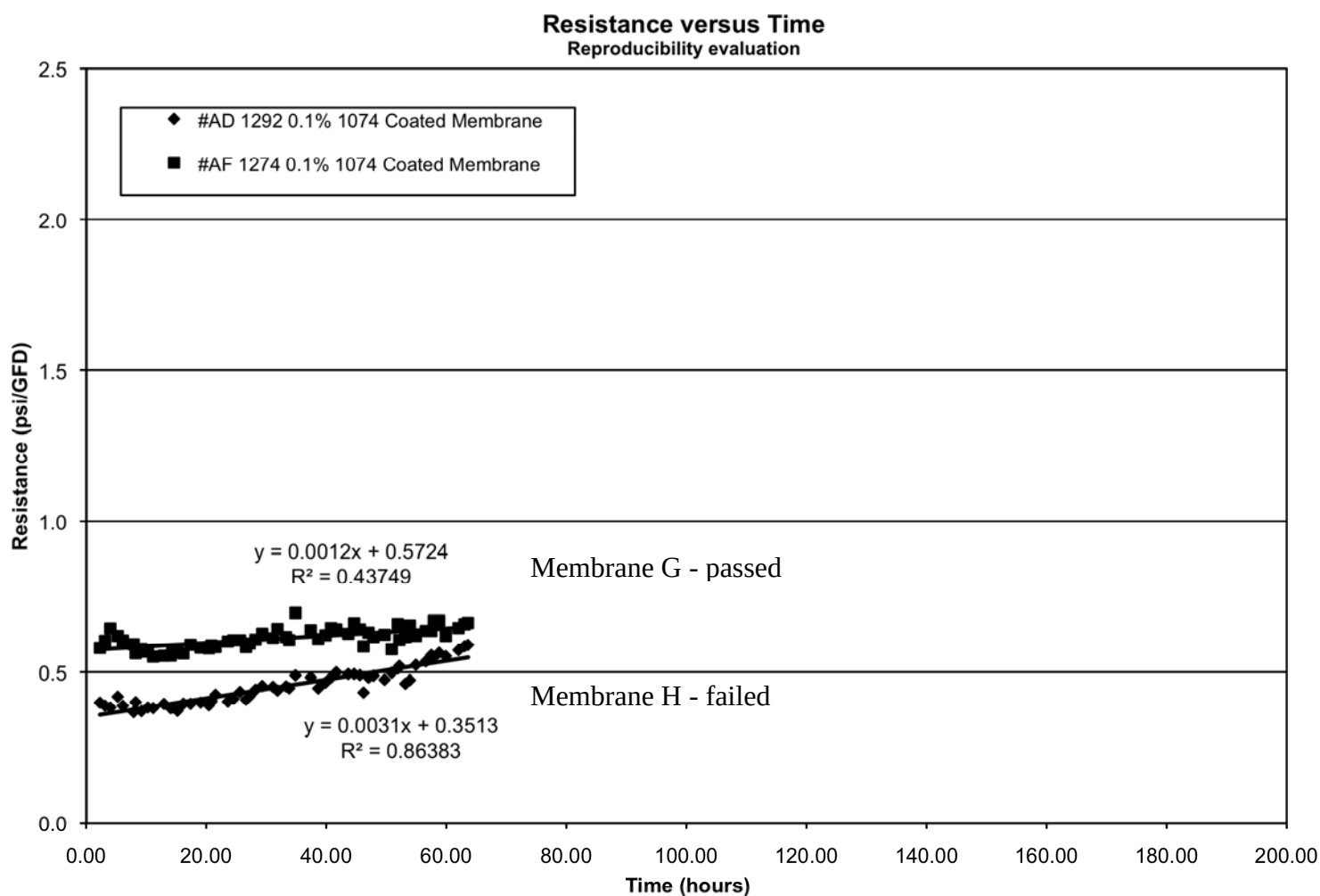
Figure 12. Membrane H, which failed, compared to Membrane G, which passed.
