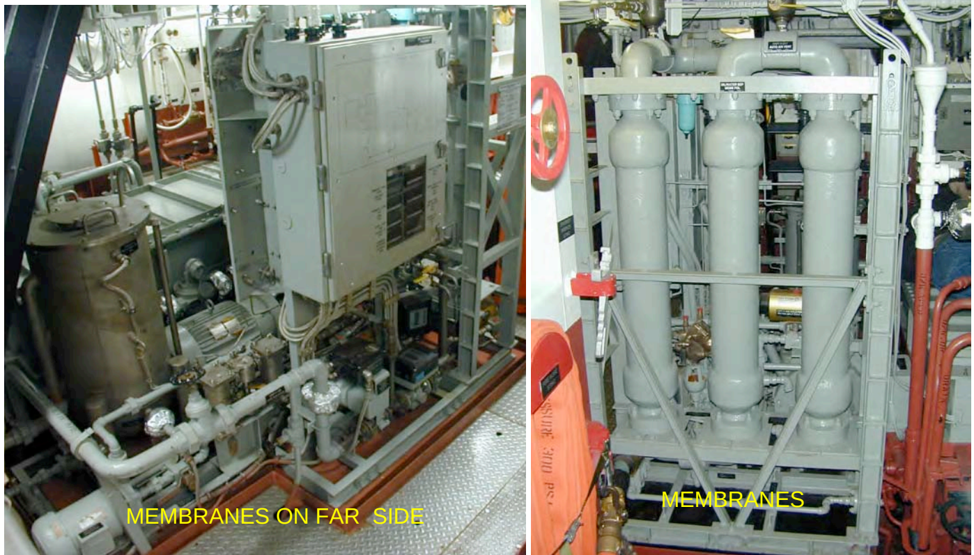
Figure 1. Oily Waste Membrane System Onboard DDG-class ship
