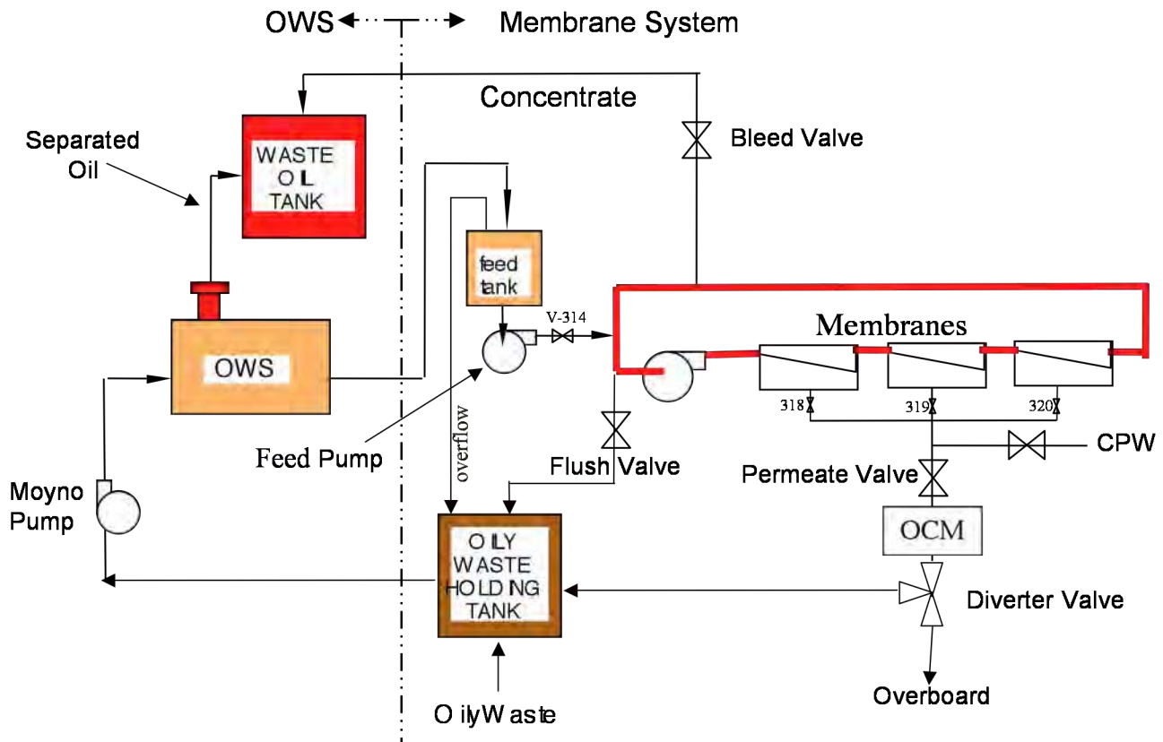
Figure 18. Basic oily waste treatment system on a Navy ship
