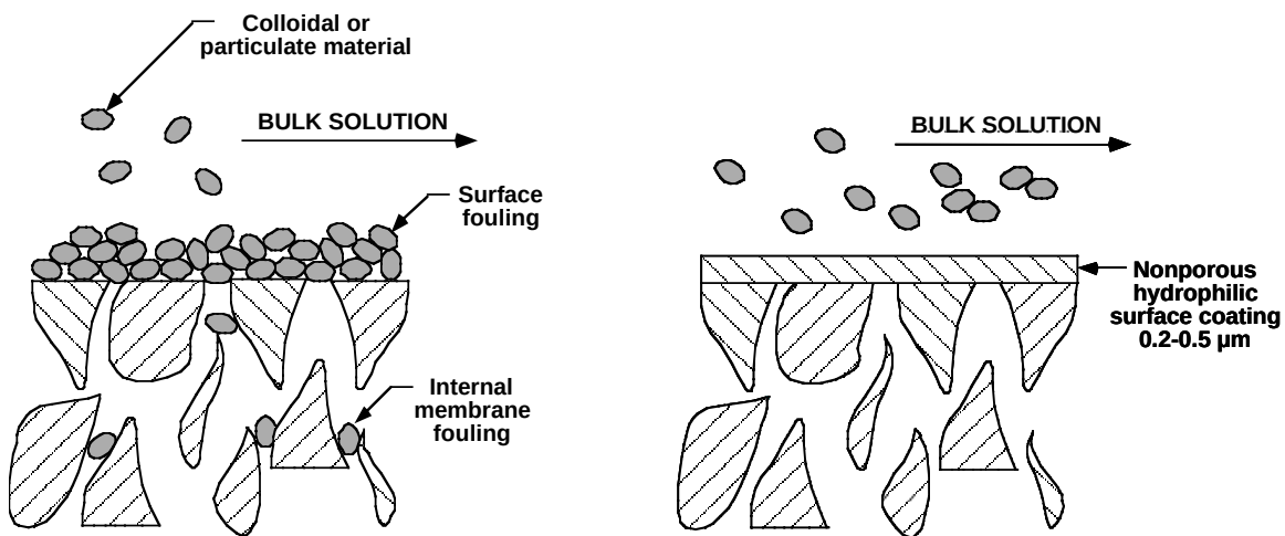
Figure 5. Membrane Surface with and without Polymer Coating
