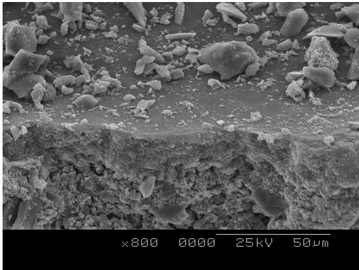
Figure 13. SEM of coated membrane surface after 120 hours of operation.
