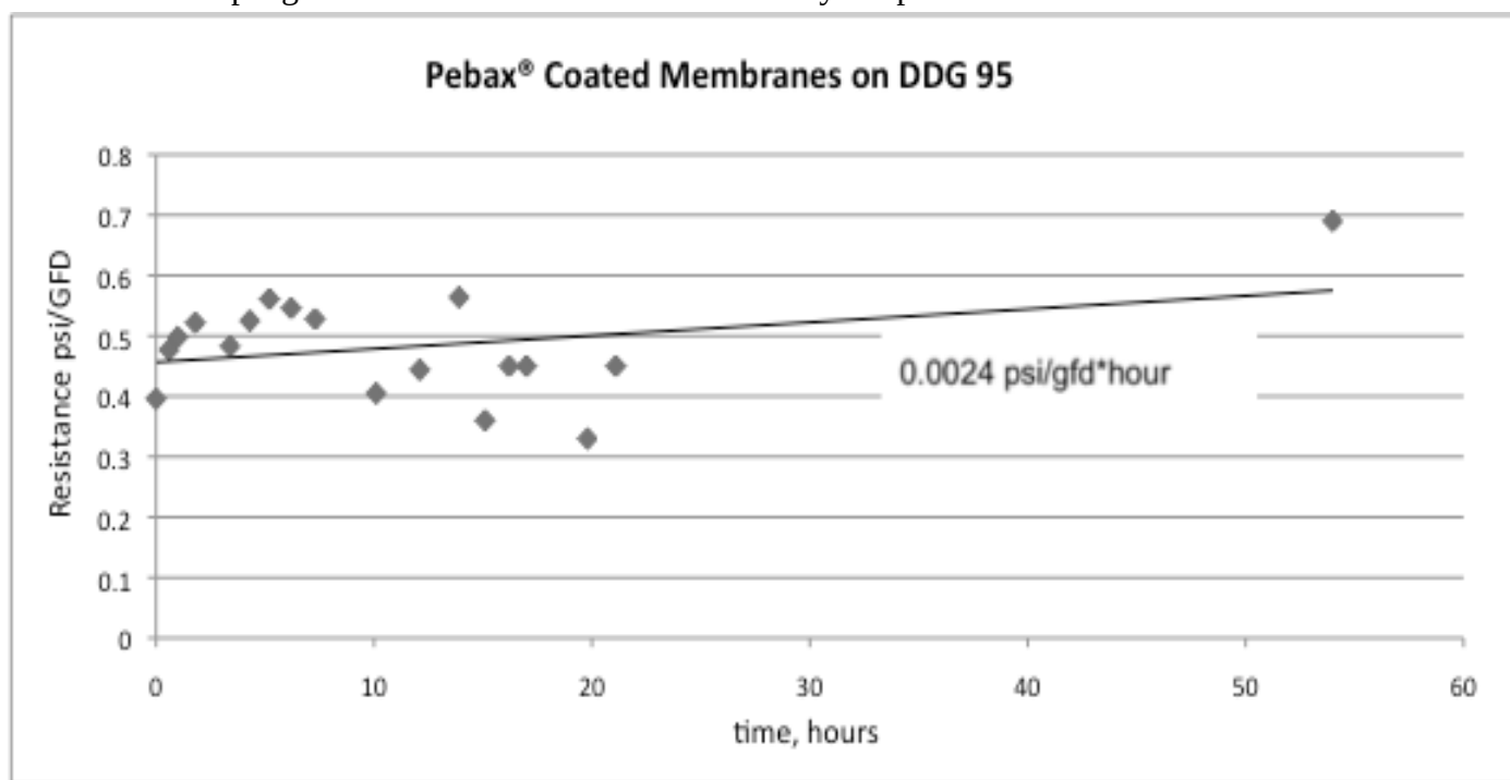
Figure 19. Shipboard Membrane Resistance of Full-Scale Coated Ceramic Membranes
