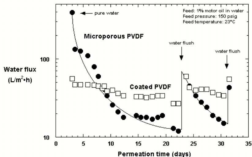
Figure 6. Water Fluxes of Coated and Uncoated Polymeric Membrane Modules as a Function of Permeation Time
