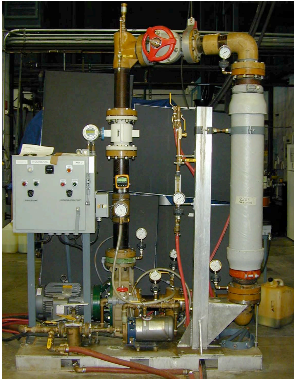
Figure 15. Full-Scale test rig.
