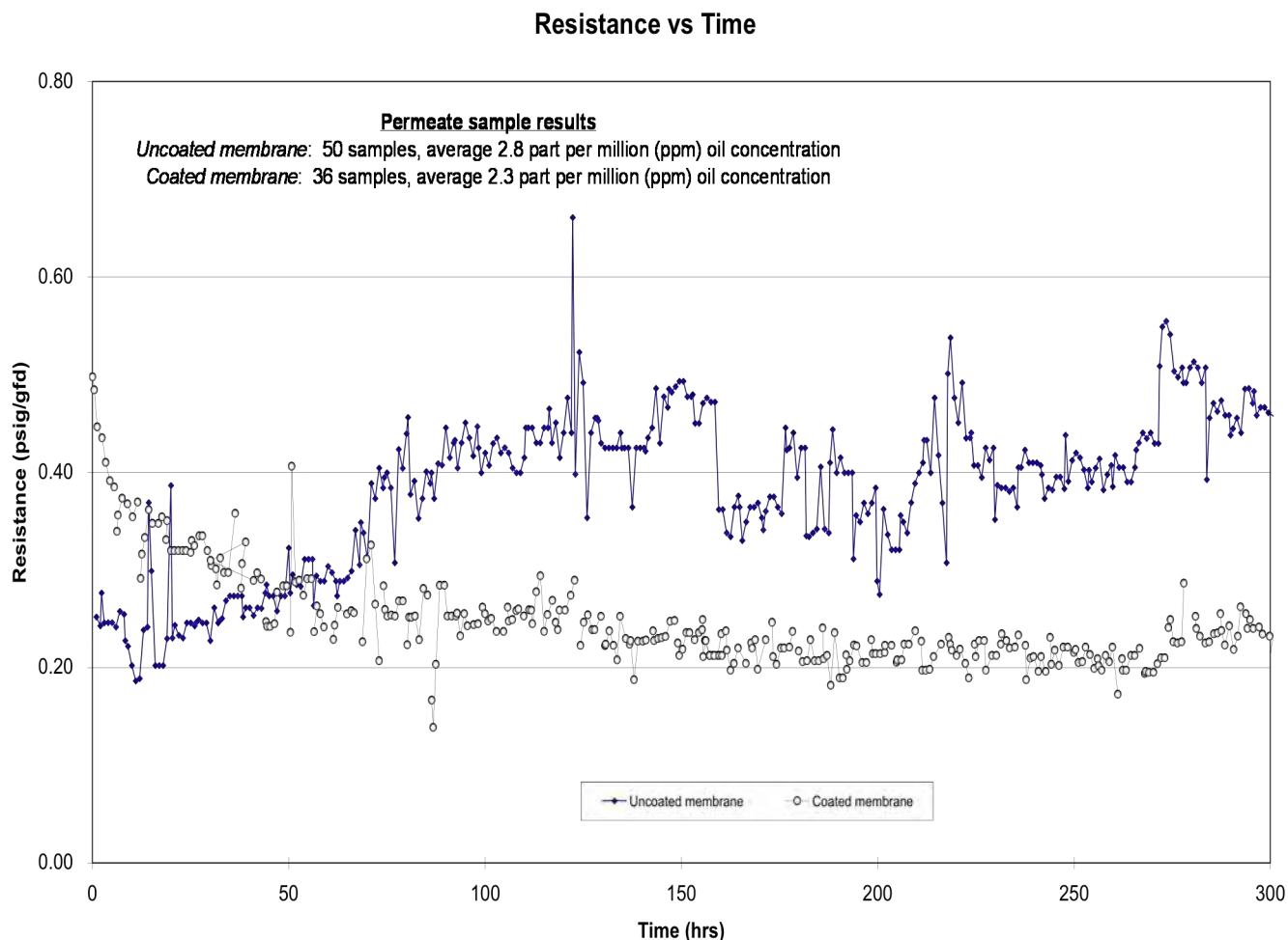
Figure 16. Resistance (psi/gfd) of full-scale membranes during laboratory test.
