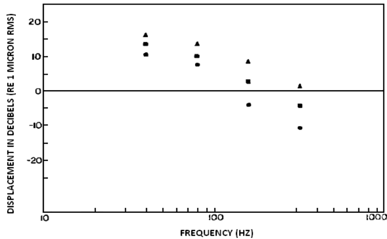
Figure A-33: Comparison of the threshold for vibration at three contactor heights. 0.5 mm below table surface (triangles), 0.5 mm above table surface (squares) and 1.5 mm above table surface (circles). Contactor area 0.113 cm 2 . Vibrations were presented to the finger. Figure taken from Verrillo (1962, p. 1770).
