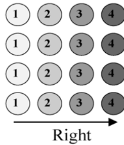
Figure 20: The pattern generated through a 4×4 array of vibrotactors for “turn right” command. The arrow represents spatial order of activation of tactors. Figure adapted from Jones et al. (2006, p. 1367).
