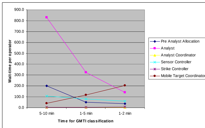
Figure 8: Wait-time per operator with decreasing time for GMTI classification
