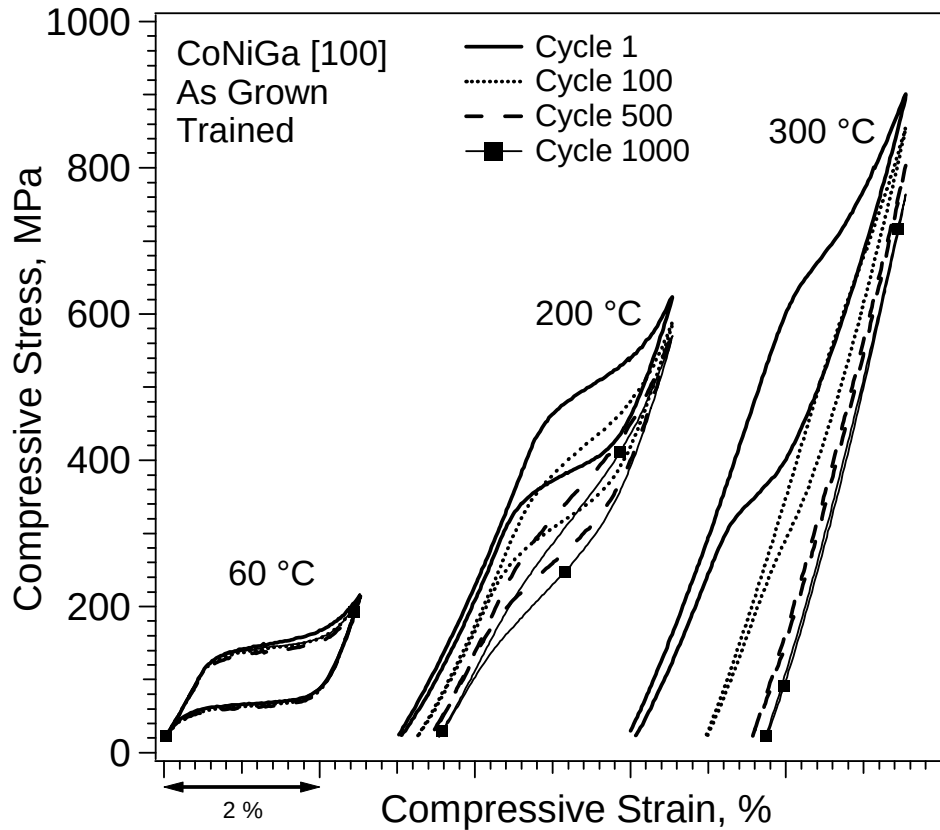
Figure 45. Cyclic deformation response of [100] oriented trained \text{Co}_{49}\text{Ni}_{21}\text{Ga}_{30} in compression at 60, 200 and 300 °C. Improved cyclic stability is observed at 200 °C while complete degradation occurs at 300 °C.
