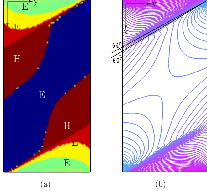
Figure 38: (a) Discriminant D at \hat{H}_y \geq 0.506 and (b) jump in the magnetic field across characteristics.
