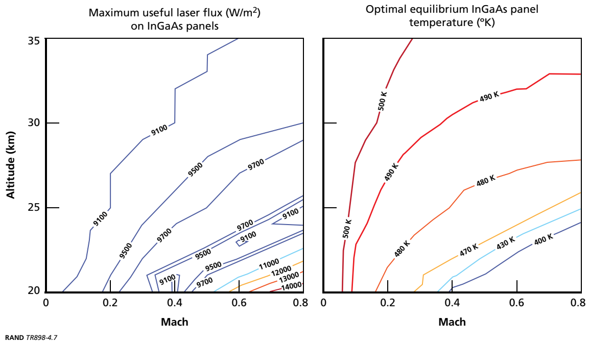
Figure 4.7 Maximum Useful Laser Flux and Resulting Equilibrium Temperature for InGaAs PVs
