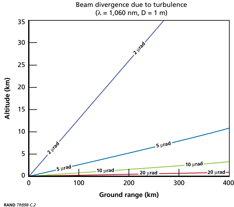
Figure C.2 Beam Divergence Caused by Turbulence for a Ground-Based Laser
