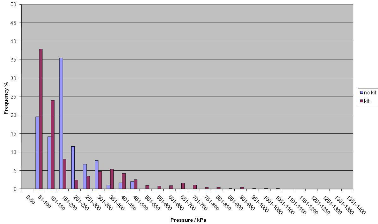
Figure 27 – Peak pressure distribution recorded for right knee during the kneeling exercise performed on grassland by Subject A.
