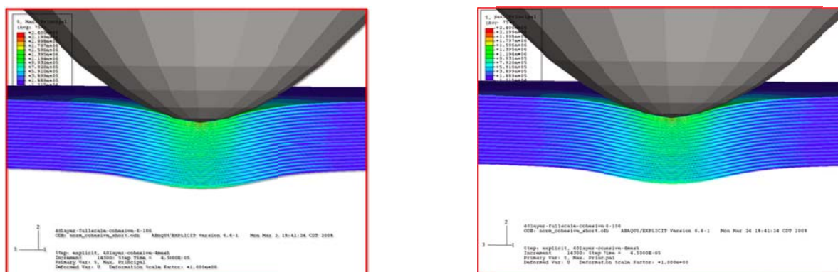
Figure 8. Deflection of the laminate (left: 0/90; right: helicoid) at 45 \mu s after impact.
