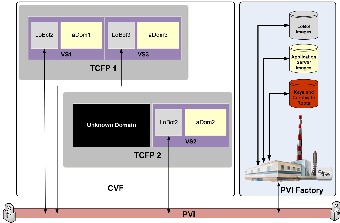
Figure 4 – PVI Architecture showing the PVI Factory and two TCFPs hosting three VSs and one unknown domain. The PVI Factory manages images and keys for the PVI and is the certificate authority.
