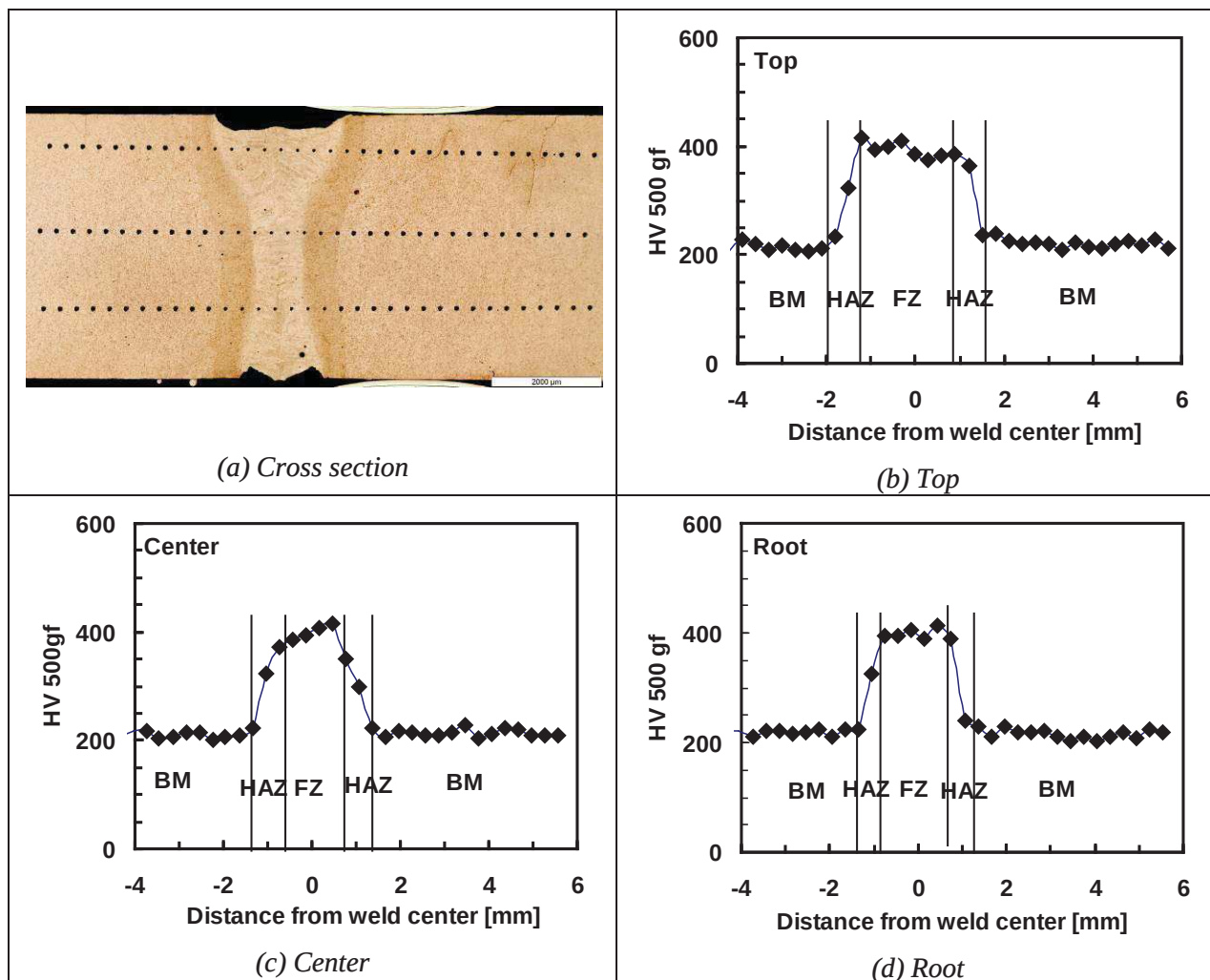
Figure 20: Hardness for Sample 2A (4 kW and 29.2 mm/s)
