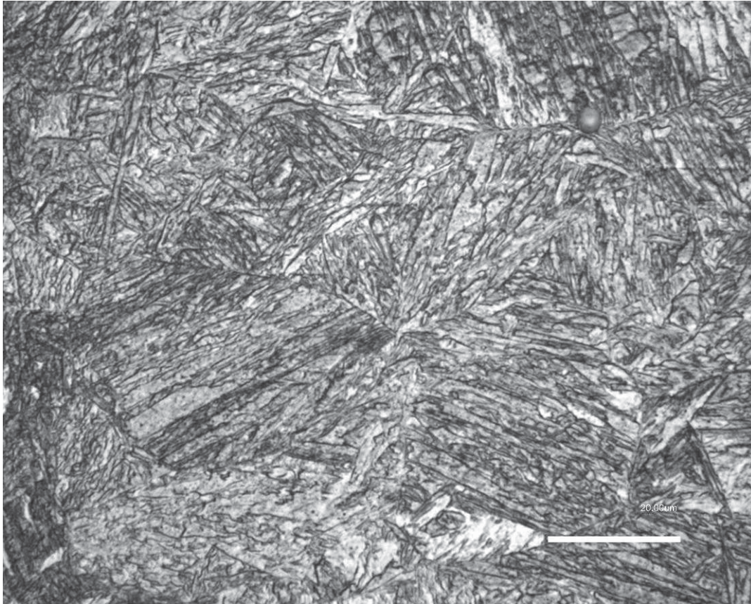
Figure 12: Fusion zone martensitic microstructure obtained from 4 kW and 29.2mm/s (137 J/mm). Scale bar represents 200 \mu m
