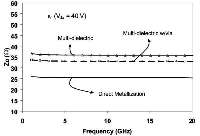
Fig. 12. Characteristic impedance Z_0 for the biased case \epsilon_r(V_{dc} = 40 \text{ V}) , comparing the direct metallization design shown in Fig. 1, the multielectric design shown in Fig. 6(a), and the multielectric with via design shown in Fig. 6(b).
