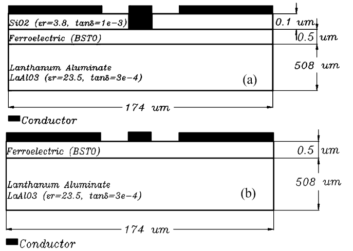
Fig. 3. (a) Cross section of ferroelectric phase shifter with the inclusion of a silicon oxide layer and the formation of a via hole under the signal conductor (b) phase shifter employing direct metallization. The metallization layers include: Cr/Ag/Au (250 Å, 14250 Å, 500 Å).
