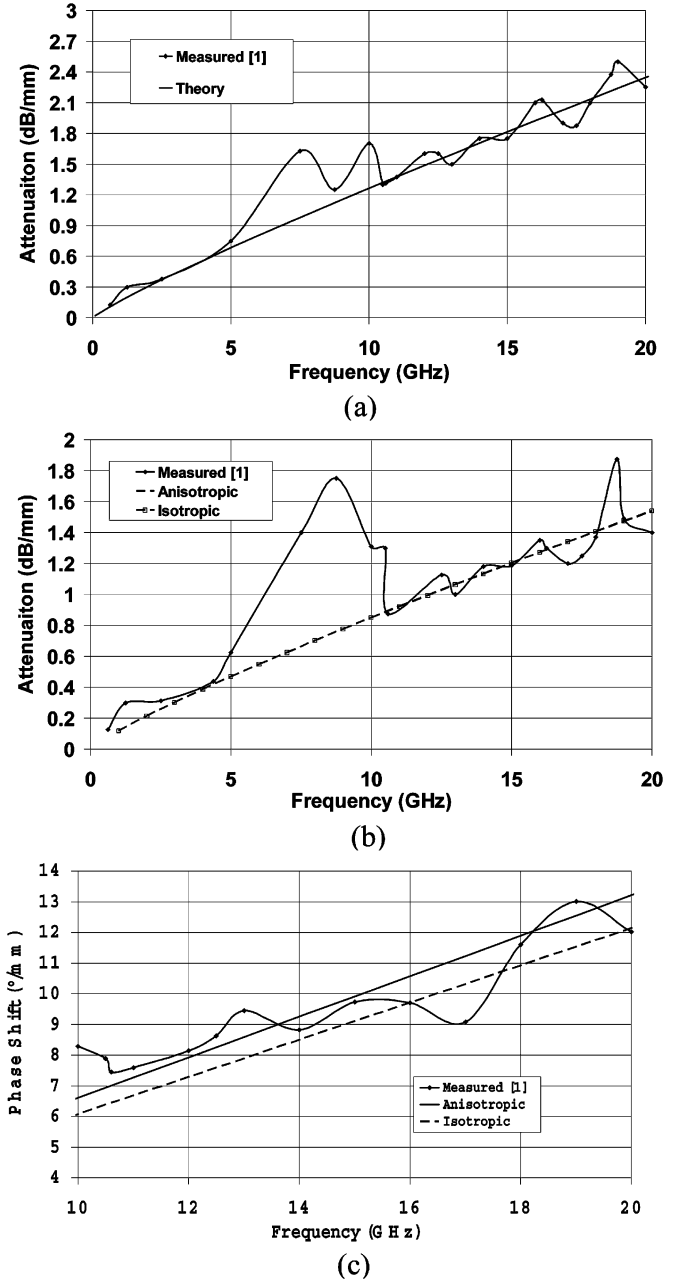
Fig. 5. (a) Attenuation constant for the unbiased case \varepsilon_r ( V_{dc} = 0 V). (b) Attenuation constant for the biased case \varepsilon_r ( V_{dc} = 40 V). (c) Phase shift versus frequency comparing experimental data to theory. The results also illustrate a comparison between anisotropic and isotropic ferroelectric permittivity representations.
