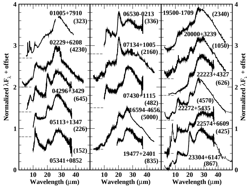
Figure 5. Plot of the normalized Spitzer IRS spectra or Infrared Space Observatory Short Wavelength Spectrometer/Long Wavelength Spectrometer (LWS) spectra for the Galactic 21 \mu\text{m} sources, along with the carbon-rich PPN IRAS 01005+7910 which lacks the feature but which is included for comparison with the LMC object J051228. As in Figure 1 the peak \lambda F_\lambda values in units of 10^{-14} \text{ W m}^{-2} are given in parentheses on the right within each panel. The spectra are generally from Hrivnak et al. (2000), Volk et al. (2002), and Hrivnak et al. (2009). The exceptions are the IRS spectrum of IRAS 01005+7910, from Cerrigone et al. (2009), plus the IRS spectra of IRAS 04296-3429 and 22223+4327 which were reduced from the Spitzer archive ( Spitzer program 00045, PI: T. Roellig). For IRAS 22574+6609 and IRAS 23304+6147, the ISO SWS/LWS spectra are shown for wavelengths not covered by the Spitzer IRS spectrum.
