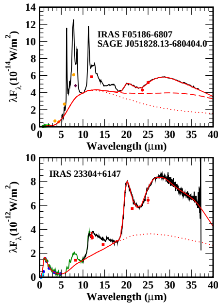
Figure 6. Top panel: the observations of object J051828 are shown as in Figure 1 with the model fit overplotted. The solid curve shows the overall model fit, the dashed curve shows the amorphous carbon continuum fit with the discrete shells to boost the continuum under the features, and the dotted curve shows the corresponding continuum fit with a smooth density distribution. Bottom panel: the Spitzer IRS and ISO PHT-S (below 10 \mu\text{m} ) spectra of IRAS 23304+6147 along with the available photometry are shown with the model fit overplotted. As in the top panel, both the full model fit and the model amorphous carbon continuum from a smooth density profile are plotted to illustrate the difference between the Galactic and Magellanic Cloud models.
