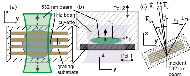
FIG. 1. (Color online) Measurement setup. (a) Top view—the terahertz radiation is incident from below the grating, normal to the page. (b) Side view— E_0 and E_\pm : electric fields of 532 nm excitation and SDFG signal; Pol 1, Pol 2: polarizer before and behind the interaction volume. (c) Wavevectors for phase matching and terahertz polarization in the plane of the grating.
