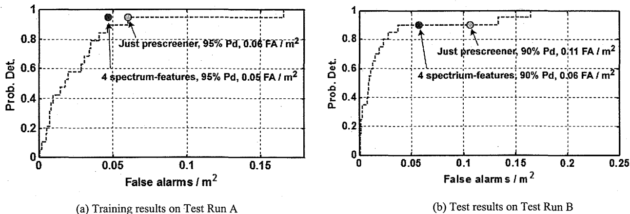
Fig. 7. Test results of one-class classifier with 4 spectrum-based features – bins [22,29,39,42] of FFT. Feature selection based on best test results. This feature selection method results in a more generalized classifier.
