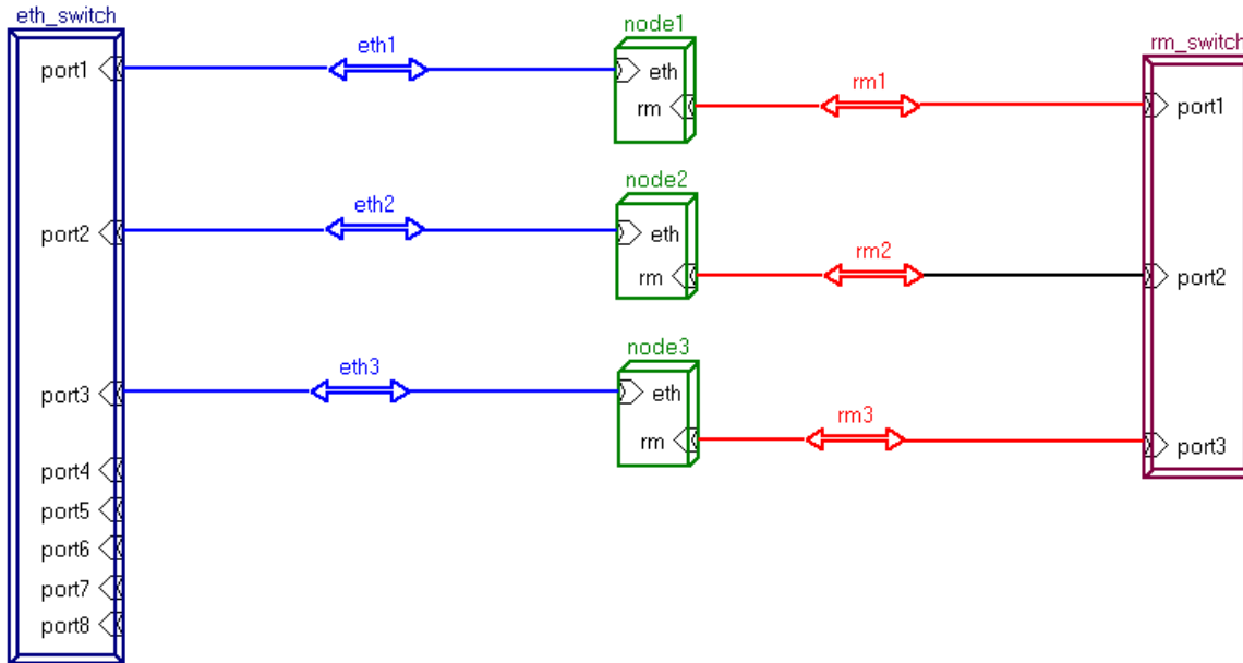
Figure 7 Hardware portion of the runtime architecture model
