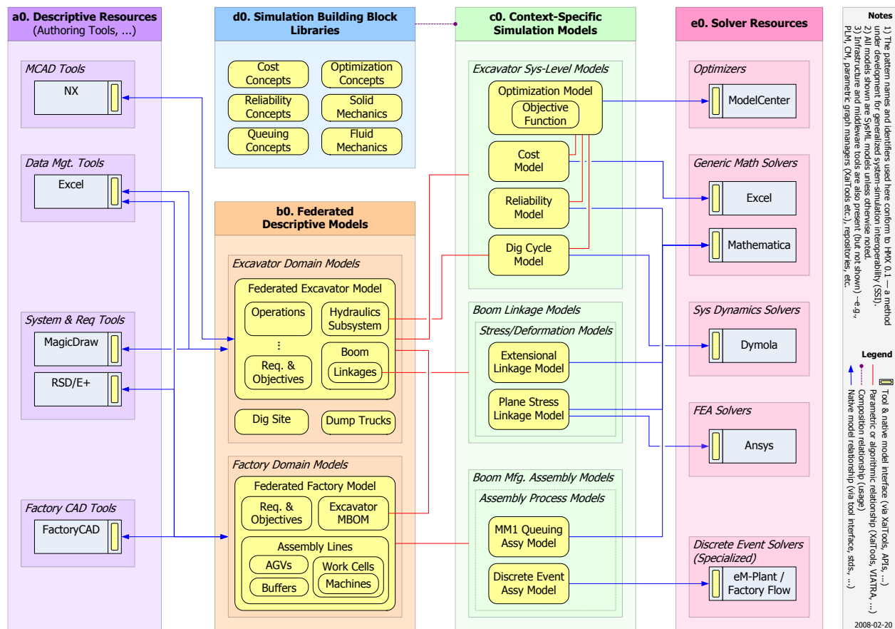
(b) Model interoperability method (MIM) patterns view (architecture view per CT-16).
