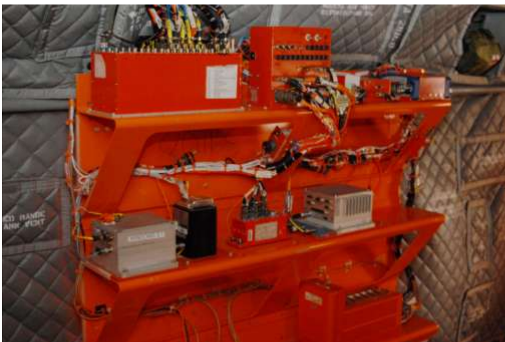
Figure 4: Picture of the STIL Stimulation Hardware
