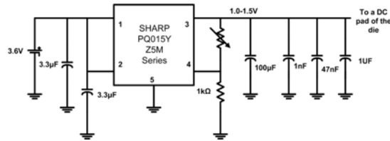
Figure A-15. DC supply regulation
