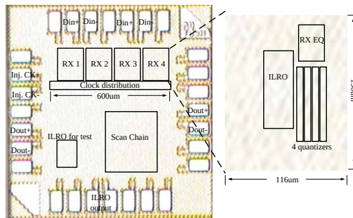
Figure 7. Die photo
