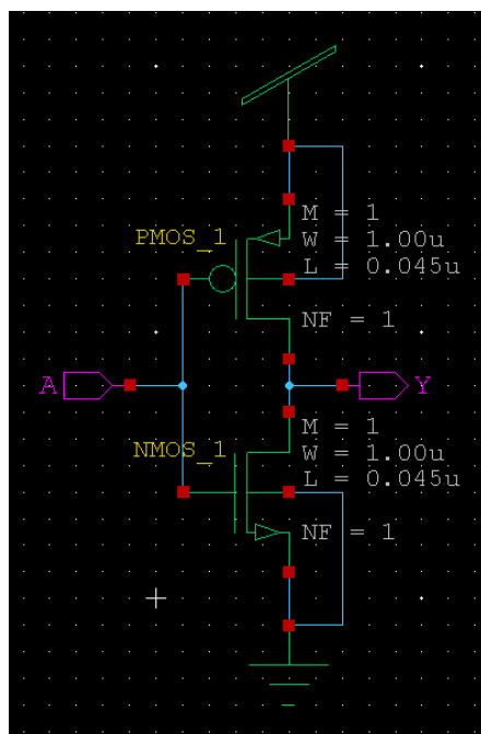
Figure 13. Tanner EDA S-Edit® view of CMOS inverter with implemented gate conduction model
