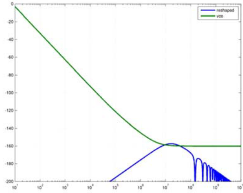
Figure 69. The DCO
