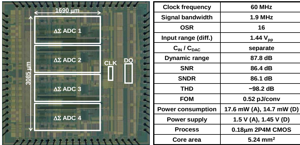
Figure 51. Die photo and summary of measured performances for self-coupled 4-cell delta sigma ADC
