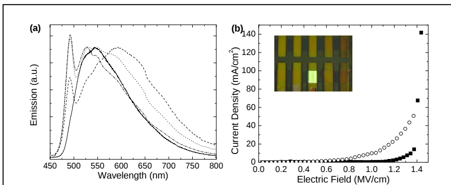
Figure 19. (a) PL emission spectra of solid state samples measured as a solution cast \text{Zn}^{2+} : 17 metallo-supramolecular polymer (dashed), spun-cast \text{Zn}^{2+} : 17 metallo-supramolecular polymer (dash-dot), spun-cast neat macromonomer 17 (dotted), and as a spun-cast metallo-supramolecular polymer \text{Zn}^{2+} : 17 LED (solid). (b) I - V curves of LEDs based on [\mathbf{17}\cdot\text{Zn}(\text{ClO}_4)_2]_n .
