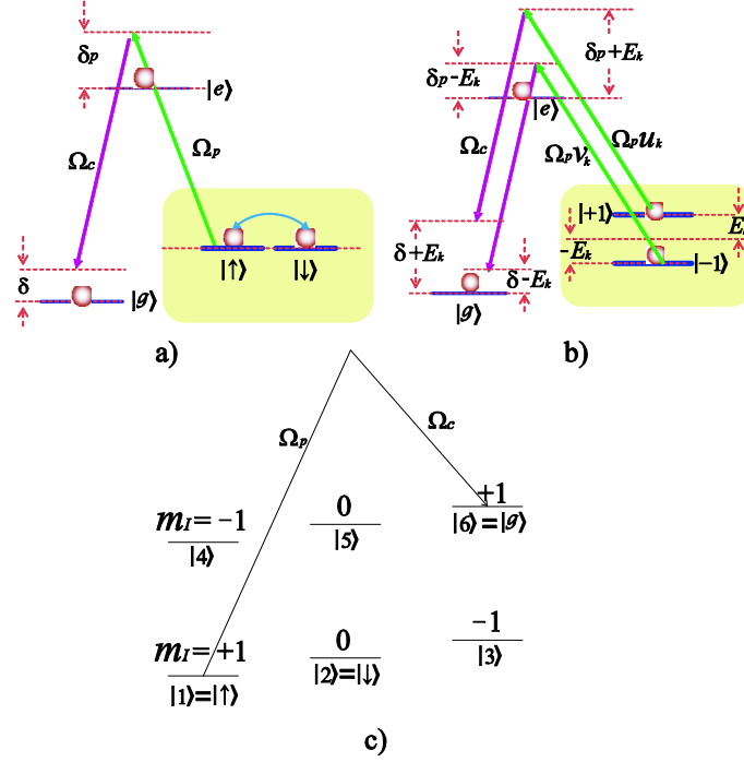
FIG. 7: (a) The bare state picture of our model. (b) The dressed state picture of our model equivalent to (a). (c) A possible realization in ^6\text{Li} . Here the states labelled by |i\rangle ( i = 1, 2, \dots, 6 ) are the 6 ground state hyperfine states. Most experiments involving ^6\text{Li} are performed with a magnetic field strength tuned near a Feshbach resonance at 834G. Under such a magnetic field, the magnetic quantum number for the nuclear spin m_I is, to a very good approximation, a good quantum number. The values of m_I are shown in the level diagrams. Two-photon transition can only occur between states with the same m_I . Any pair of the lower manifold ( |1\rangle , |2\rangle , and |3\rangle ) can be chosen to form the pairing states. In the example shown here, we choose |1\rangle = |\uparrow\rangle , |2\rangle = |\downarrow\rangle and |6\rangle = |g\rangle . The excited state |e\rangle (not shown) can be chosen properly as one of the electronic p state.
