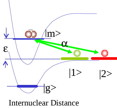
FIG. 2: The schematic of a coupled two-species atom-heteronuclear-molecule condensate system involving a Feshbach resonance.
