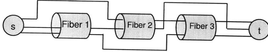
Figure 2-1: A logical topology with 3 links where each pair of links shares a fiber in the physical topology.
