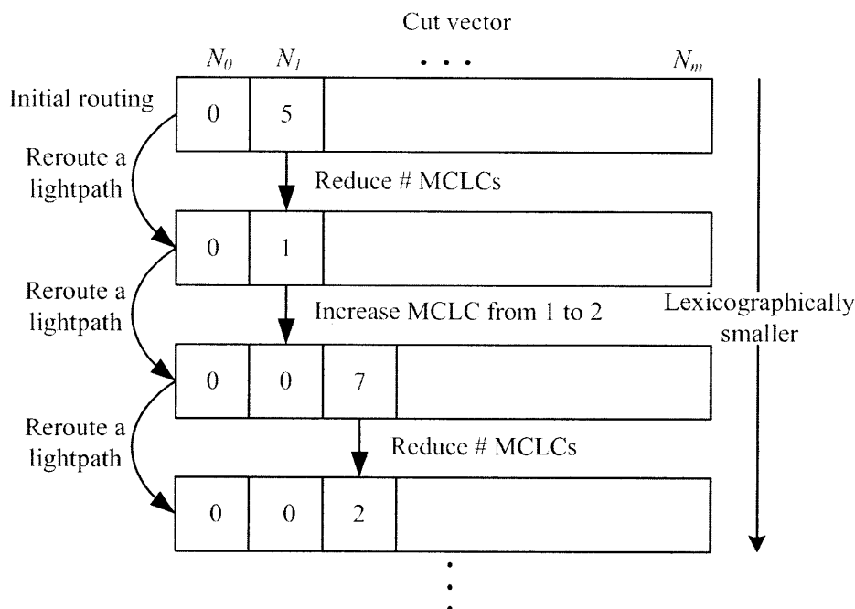
Figure 5-2: The lightpath rerouting framework.
