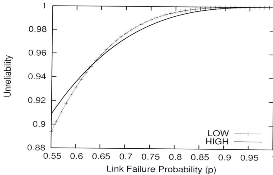
(c) Unreliability of the two Lightpath Routings
