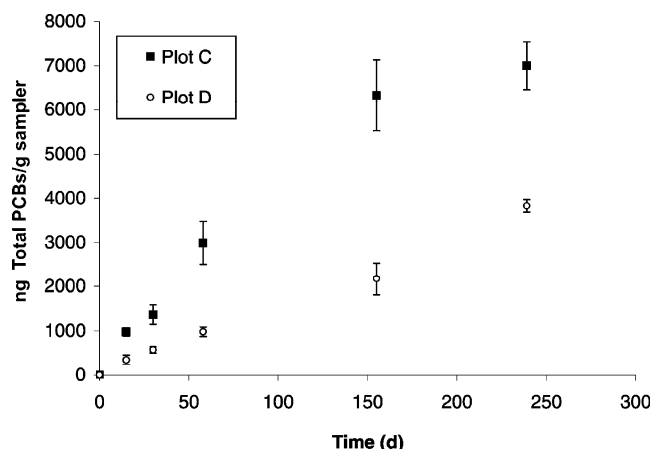
Figure 14. Uptake of PCBs over time in PEDs deployed in sediment in mixed-only Plot C (squares) and activated carbon amended Plot D (circles) at Hunters Point, San Francisco, CA ( n = 3 ).
