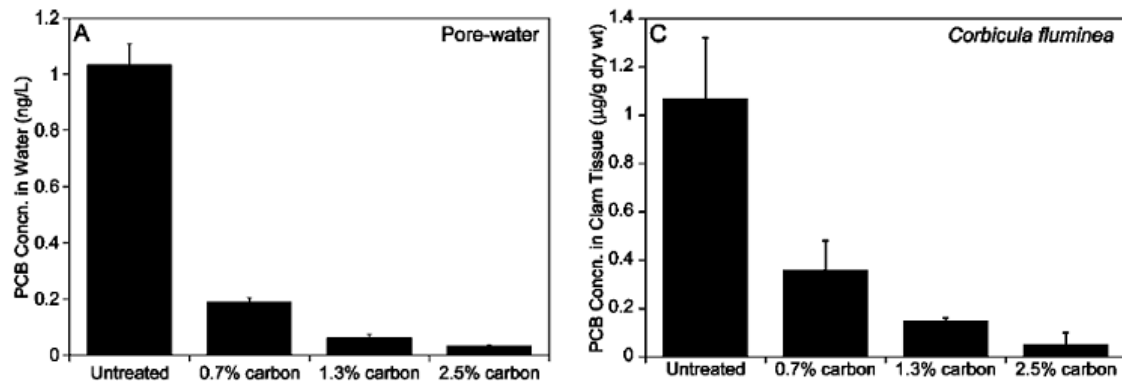
Figure 24. PCB concentrations in water (left) and clam tissue (right) after exposure to untreated sediment and sediment amended with different doses of activated carbon (McLeod, Luoma et al. 2008).
