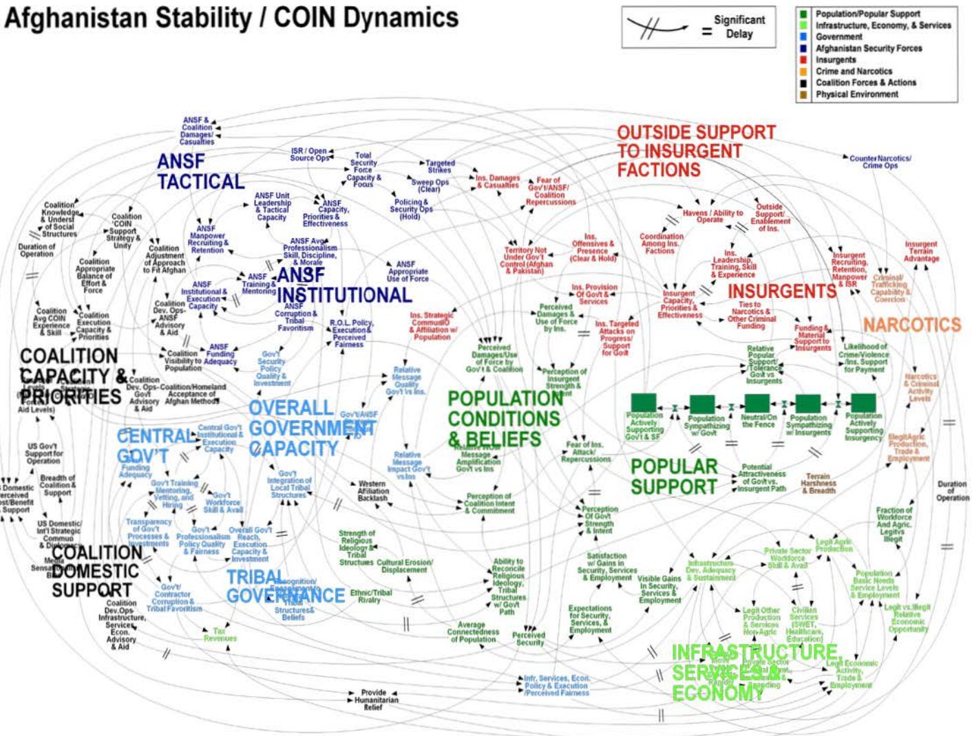
Figure D-1: Afghanistan Stability and Counter-Insurgency Dynamics Model 1
