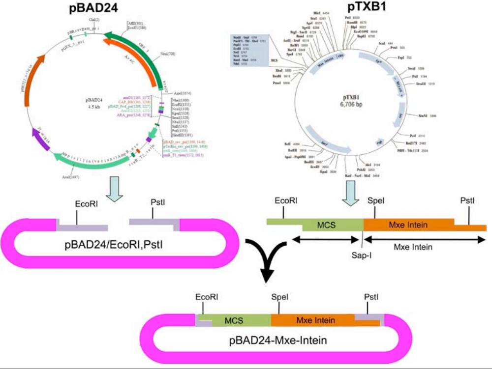
Figure 5. Scheme used for the cloning of cyclotide-based libraries using the pBAD24 (Arabinose driven promoter) and pTXB1 (T7-driven promoter) derived expression vectors.
