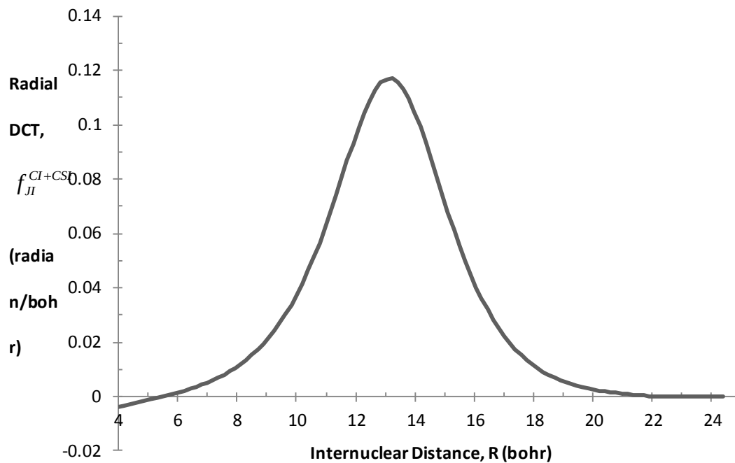
Figure 32. Radial DCT between \Pi_{\frac{1}{2}} and \Sigma_{\frac{1}{2}} states
