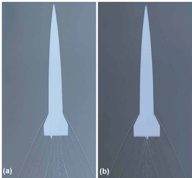
Fig. 24 Horizontal shadowgraphs for shot 24 096 at stations (a) 295 and (b) 300
