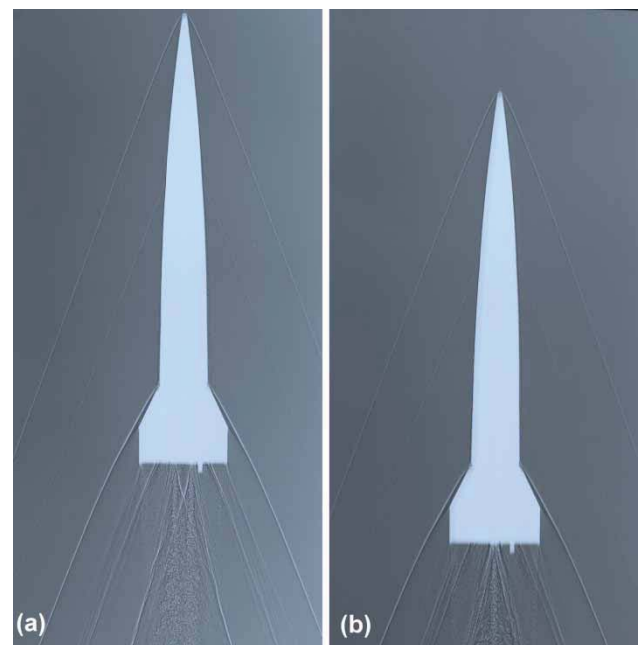
Fig. 23 Vertical shadowgraphs for shot 24 096 at stations (a) 22 and (b) 27
