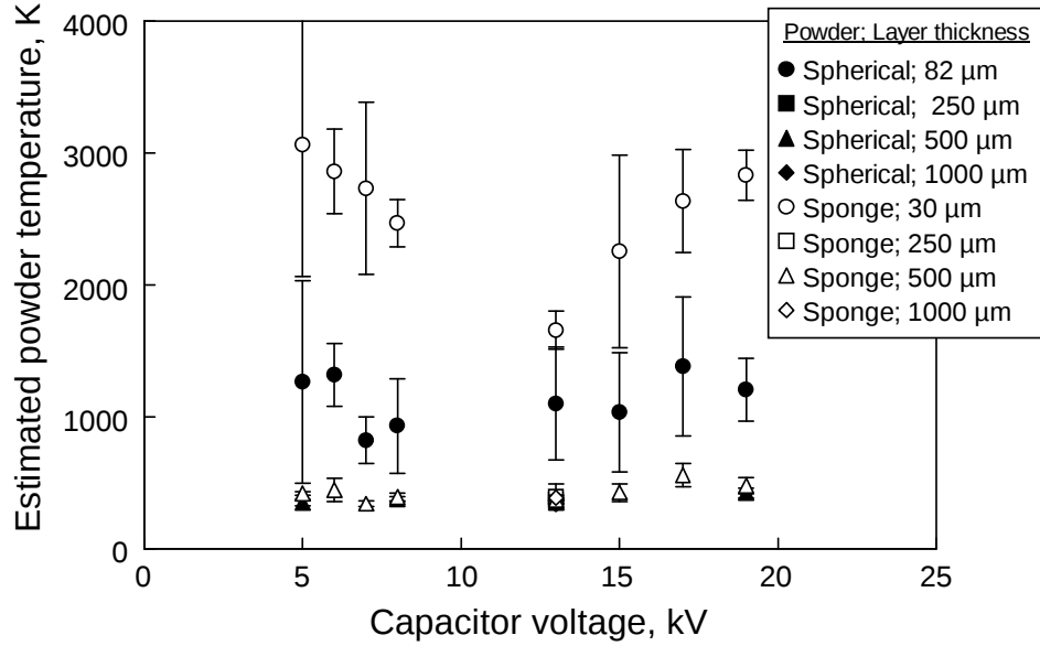
Figure 5.19 Powder temperatures estimated using Eq. (3) and assuming that the radius of the heated powder cylinder is equal to that of the spark imprint. The depth of the heated powder volume is shown in legend and is assumed to be equal to the entire thickness of the sample tested.
