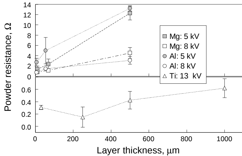
Figure 6.5 Powder resistance as a function of the powder sample thickness for different powders. ESD voltage is shown in legend.
