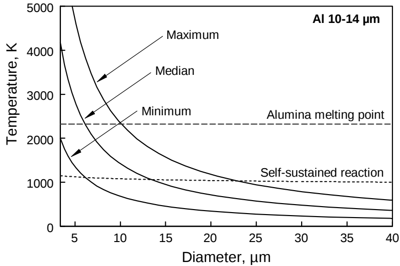
Figure 4.11 Solid lines show temperatures of particles heated by the spark as a function of their diameter based on Eq. 3 for Al 10-14 \mu\text{m} for three spark energy levels. Dashed lines show temperatures for which ignition criteria are satisfied (see text).
