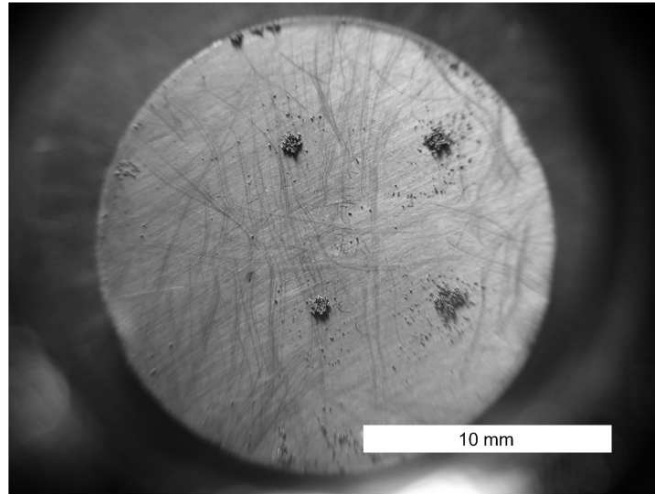
Figure 5.1 Optical microscope image of fused spherical Ti particles formed in a 0.5-mm thick sample placed in a brass sample cup.
