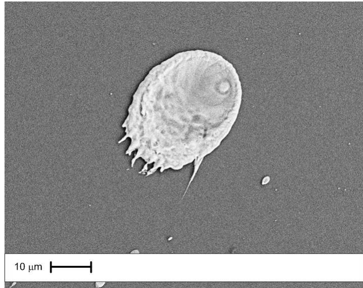
Figure 5.17 SEM image of a close-up of a molten Ti droplet.
