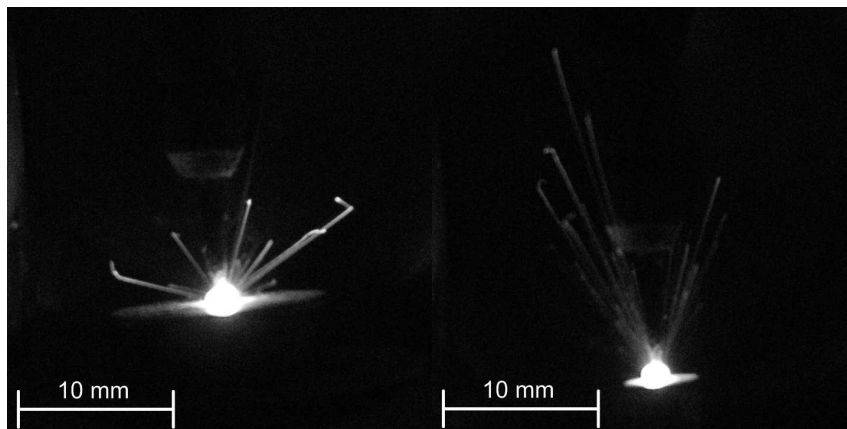
Figure 6.10 Images of the individual particle streaks produced by Al powder ignited by 12-kV ESD when the powder was prepared as a 500 \mu\text{m} -thick layer (left) and 54.1 \mu\text{m} -thick layer (right).
