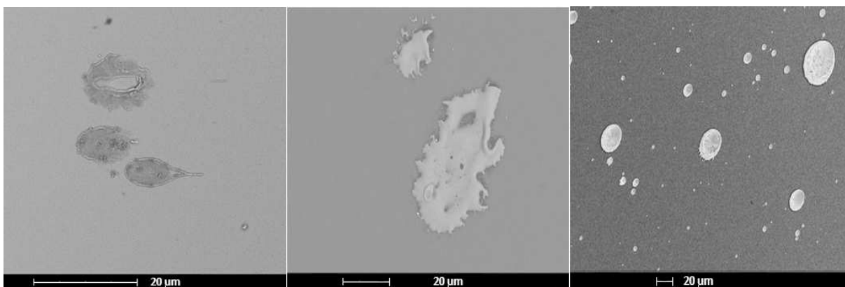
Figure 6.13 SEM image of captured particles ejected from the powder monolayer struck by spark in Ar: left to right: Mg, Al, Ti.
