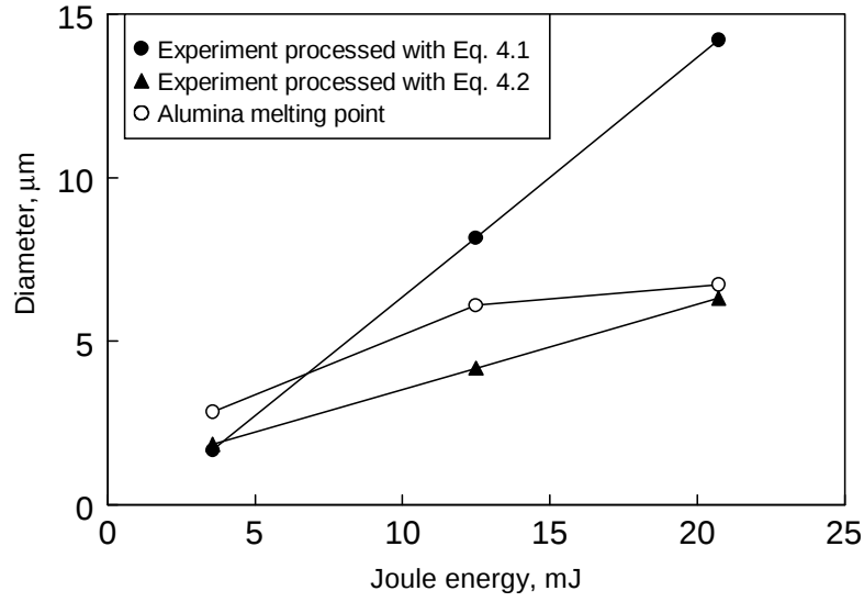
Figure 4.12 Filled symbols show diameters of the largest ignited particles obtained from experimental burn times and correlations (Eq. 4.1) and (Eq. 4.2). Open symbols show particle diameters predicted to be heated to the alumina melting point for different Joule heat energies. All processing is based on results for Al 10-14 \mu\text{m} powder.
