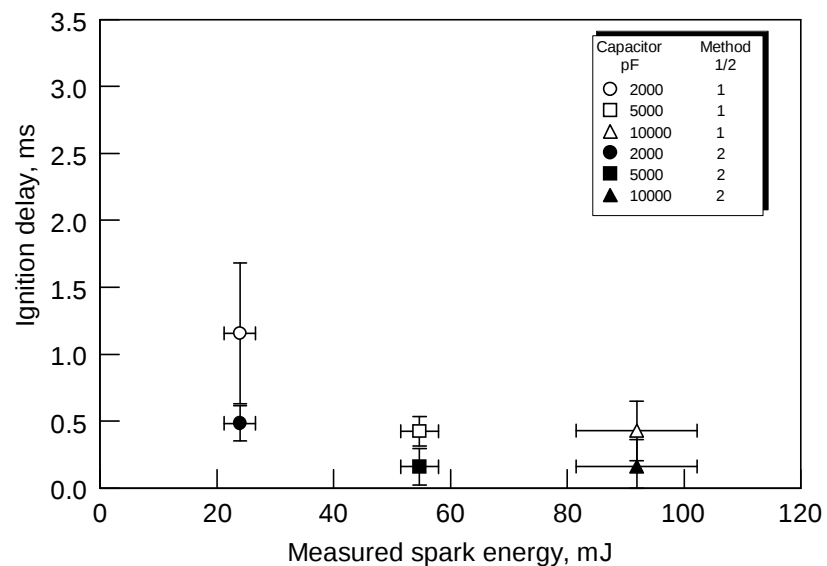
Figure 3.13 Ignition delay (both methods) as a function of the measured spark energy for experiments conducted with the 2.1 mm diameter sample holder and no binder at 8 kV and a gap of 0.2 mm.
