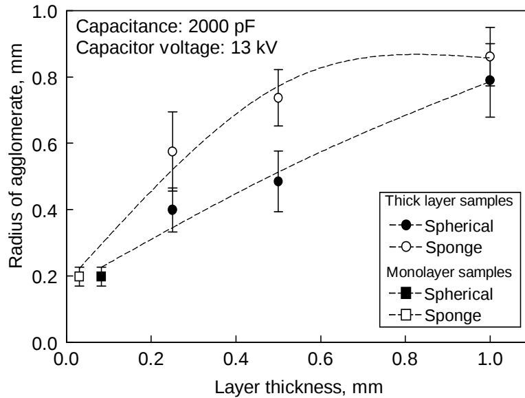
Figure 5.7 Agglomerate radius of fused Ti particles as a function of powder layer thickness for spherical and sponge powders at a capacitance of 2000 pF and a capacitor voltage of 13 kV.
