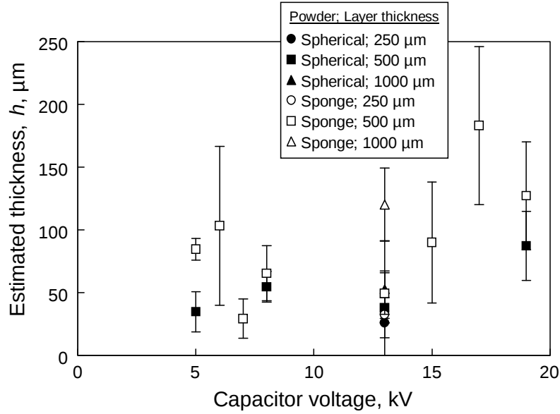
Figure 5.20 Estimated powder layer depths, h , expected to be heated to 1000 K by ESD using Eq. (5.2) solved for h and using T=1000 K. The depth of the actual powder sample is shown in legend.
