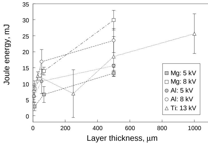
Figure 6.7 Powder resistance as a function of ESD voltage. Powder sample thickness is shown in legend.
