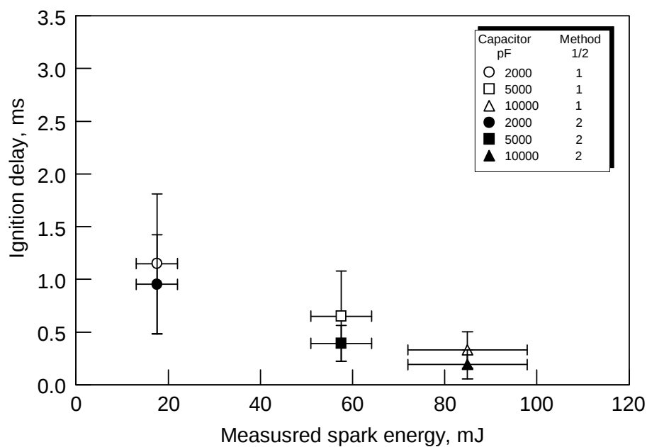
Figure 3.14 Ignition delay (both methods) as a function of the measured spark energy for experiments conducted with the 6 mm diameter sample holder and binder at 8 kV and a gap of 0.2 mm.
