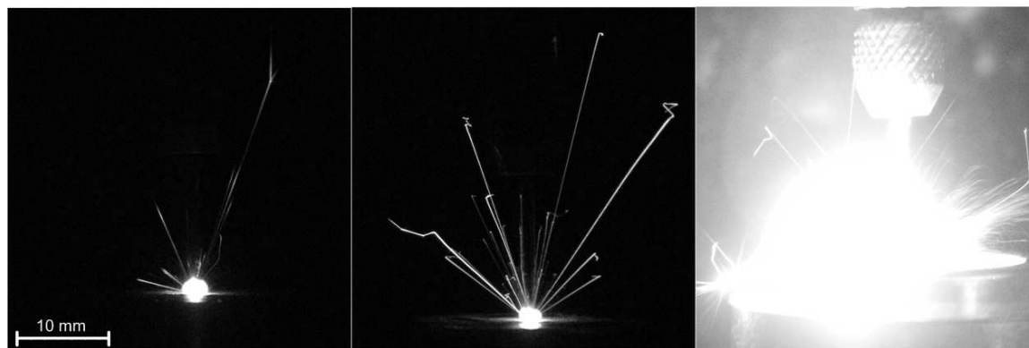
Figure 4.4 Images of streaks produced by the sparks striking an empty steel sample holder (left), and sample holder filled with 3-4.5 \mu\text{m} Al powder (center and right). All images were taken at a voltage of 8 kV.
