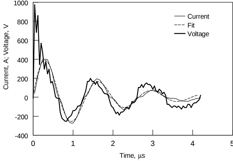
Figure 3.4 Experimental current and voltage traces for a spark and a current trace obtained fitting the experimental data and assuming the spark as a series LRC circuit.
