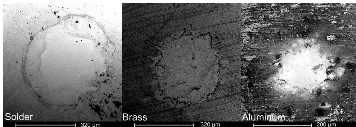
Figure 4.1 SEM images of spark spots striking solder (left), brass (middle), and aluminum (right).
