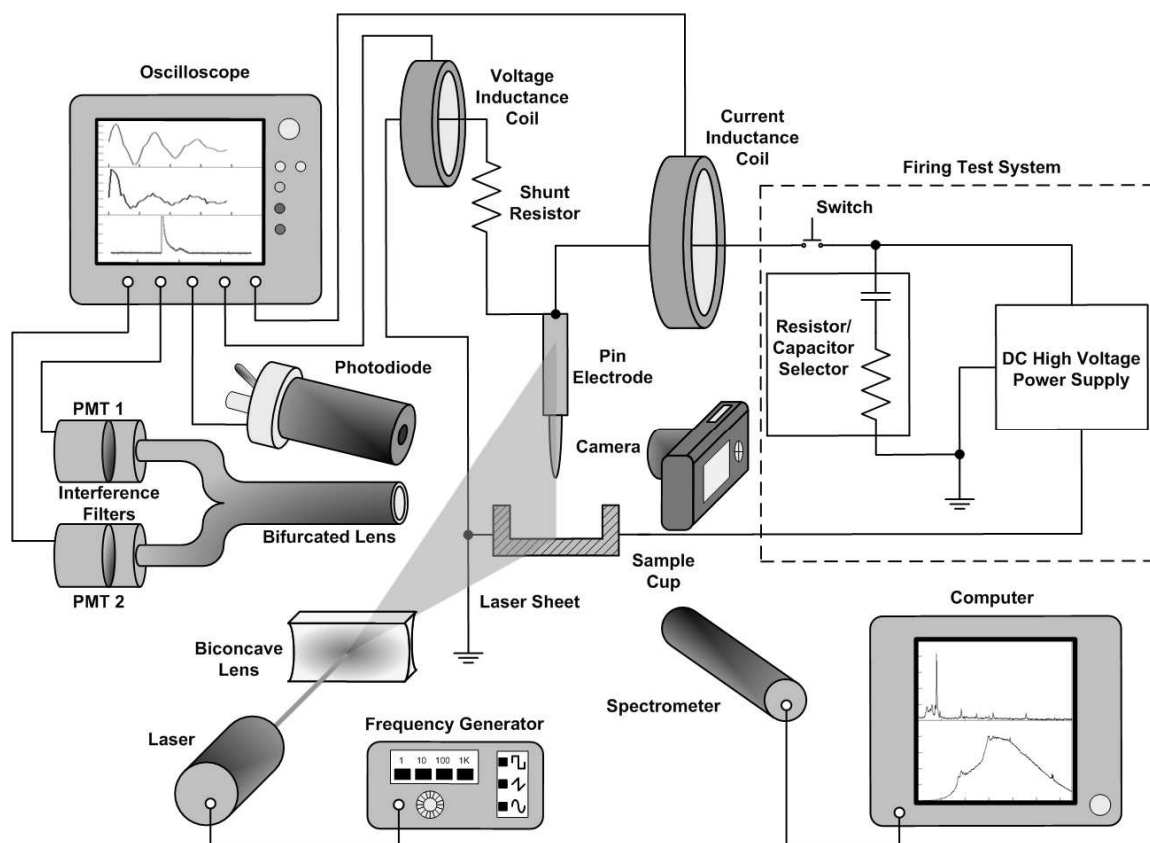
Figure 2.1 Schematic diagram of the experimental setup.
