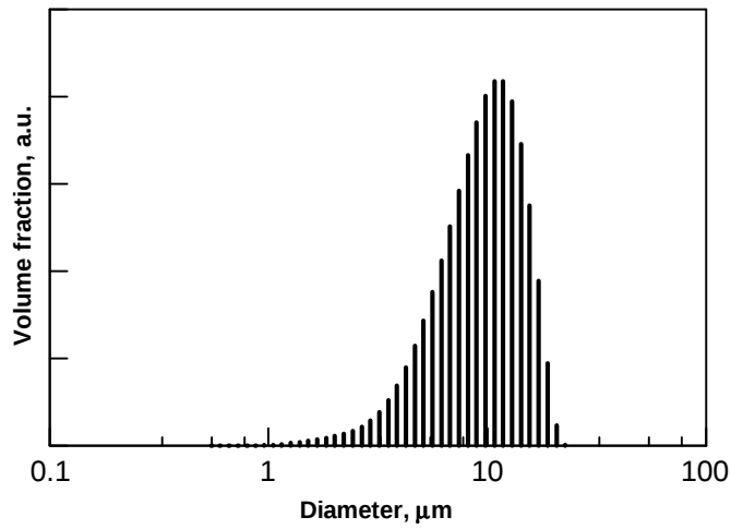
Figure 2.4 Particle size distribution of spherical Mg powder used in experiment having a mean particle size of 10.3 \mu\text{m} .
