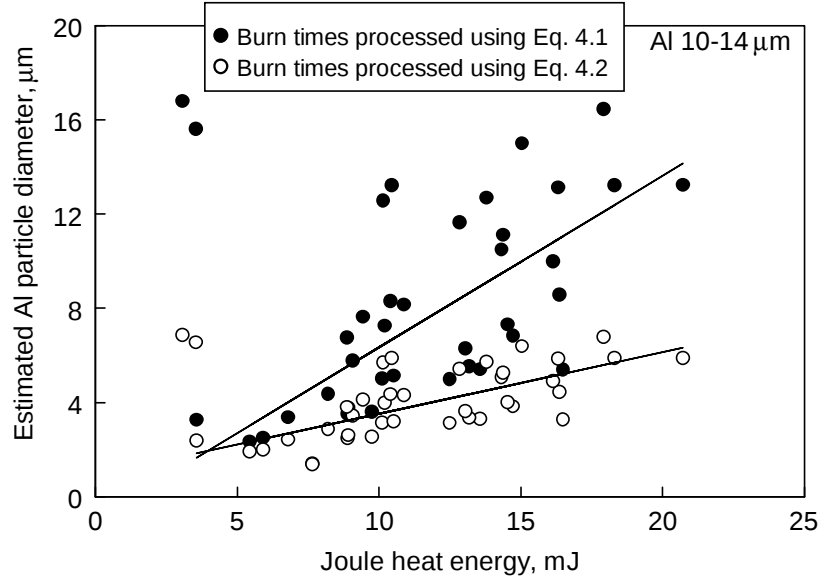
Figure 4.9 Estimated particle diameters based on expressions Eq. 4.1 and Eq. 4.2 as a function of the Joule heat energy for Al 10-14 \mu\text{m} (from data shown in Fig. 4.8).
