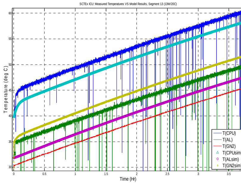
Figure 5.27: SCTEx ICU Temperature Profile, Measured Vs. Simulated, 13W/20C
