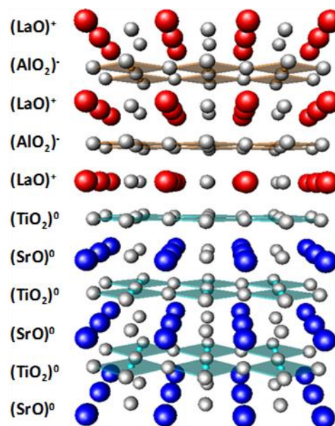
Figure 1. Oxide heterostructure consisting of 3 unit cells of polar \text{LaAlO}_3 grown on \text{TiO}_2 -terminated (non-polar) \text{SrTiO}_3 . The polar discontinuity supports the formation of a conducting interface when the top \text{LaAlO}_3 surface is positively charged. Adapted from Ref. [9].
