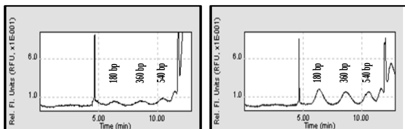
Control (0.125% DMSO)
