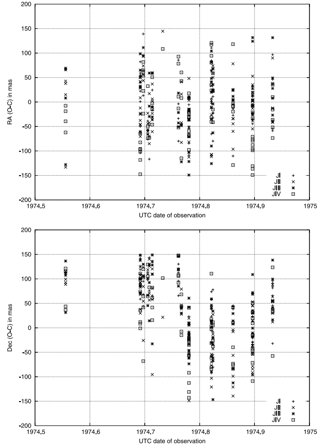
Figure 9. (RA, Dec.) (O–C) according to the DE421 theory and with DAMIAN digitizations: USNO Galilean plates of 1974.
