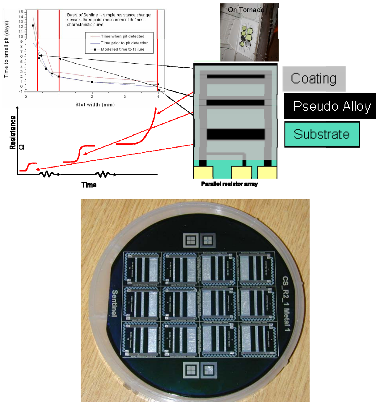
Figure 6-39: Sentinel Coating Degradation Sensor by BAE Systems. Indicates breakdown of protection scheme, onset of corrosion, and progress of corrosion. Fitted to Tornado, selected by JSF, and fitted onto MOD UK land-based assets.
