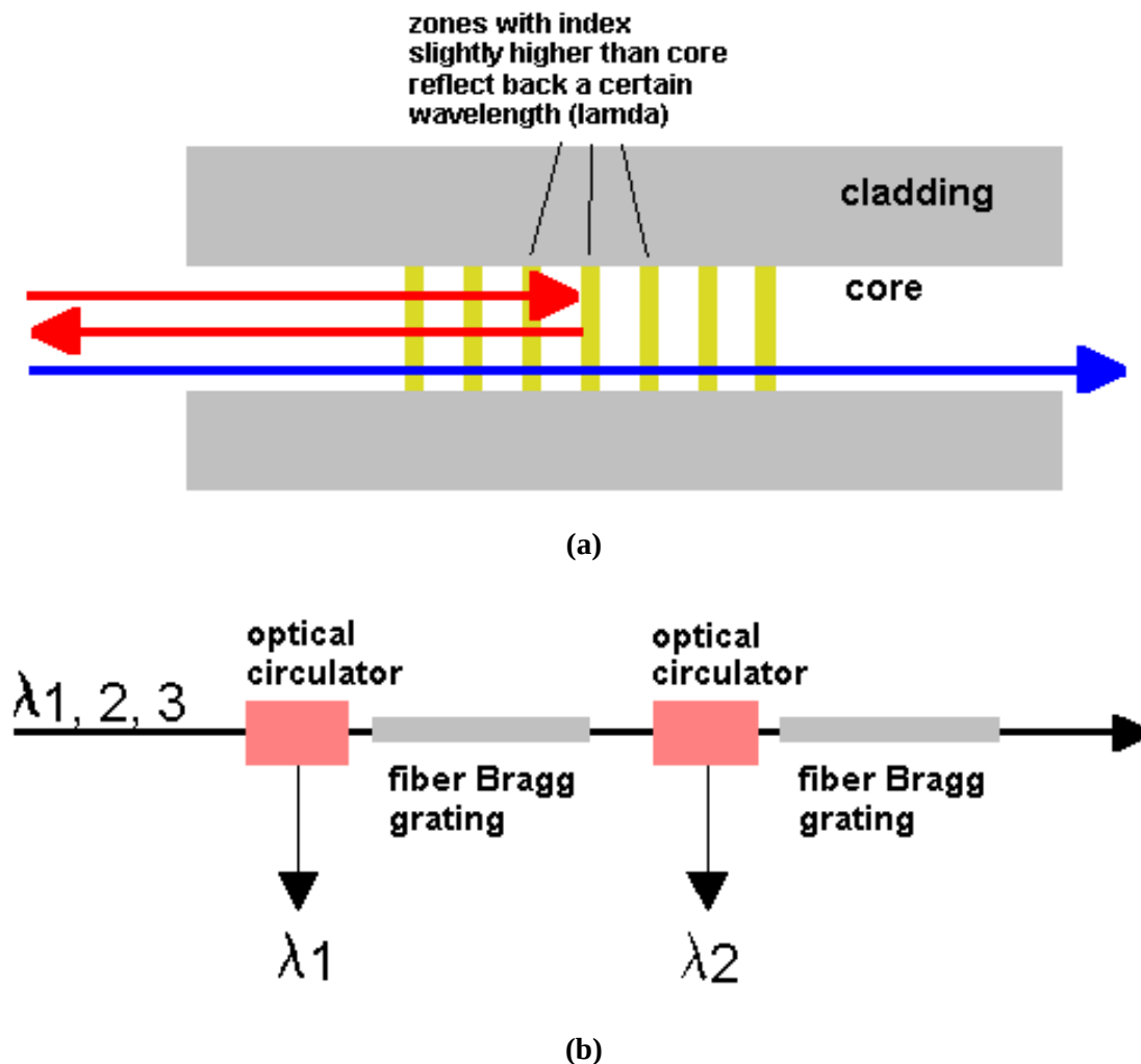
Figure 6-29: Fibre Bragg Gratings Principle of Operation.
