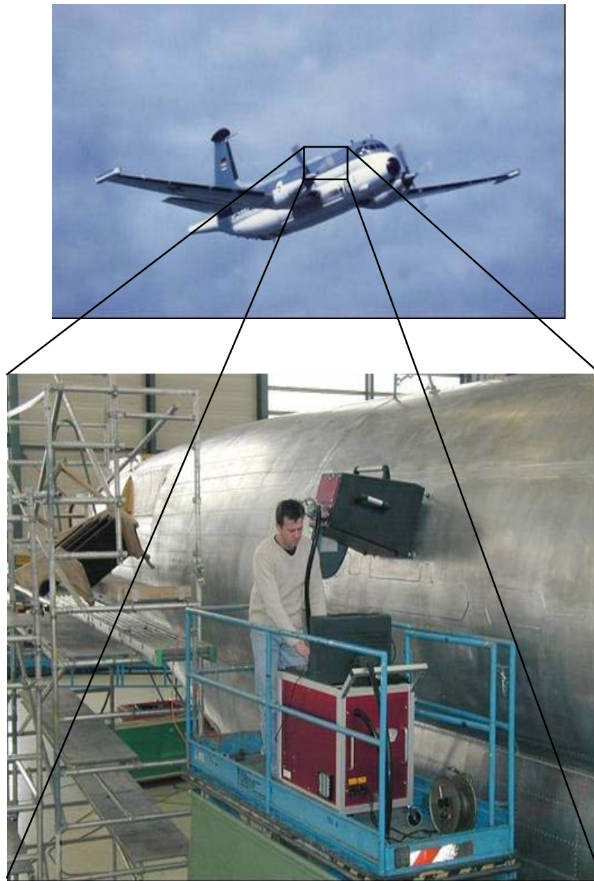
Figure 6-19: Breguet Atlantic Aircraft – Detection of Debonding in Honeycomb Structure in the Fuselage and Wing.
