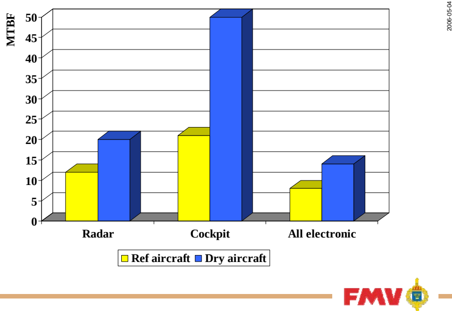
Figure 6-106: Effect of Dehumidification on MTBF.
