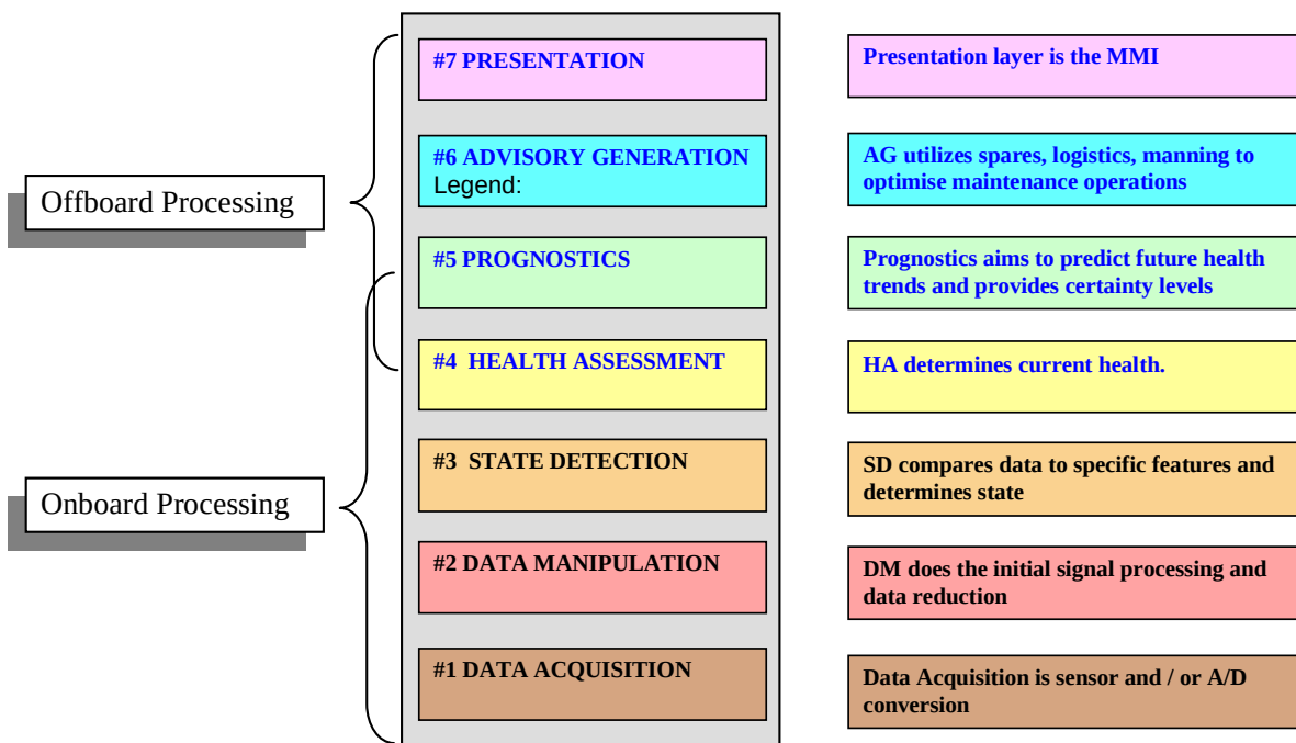
Figure 6-68: OSA-CBM.
