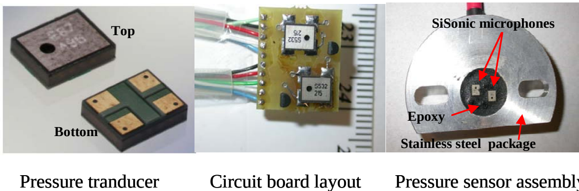
Figure 6-23: MEMS-Based Pressure Sensor for Gas Turbine Engine Applications.
