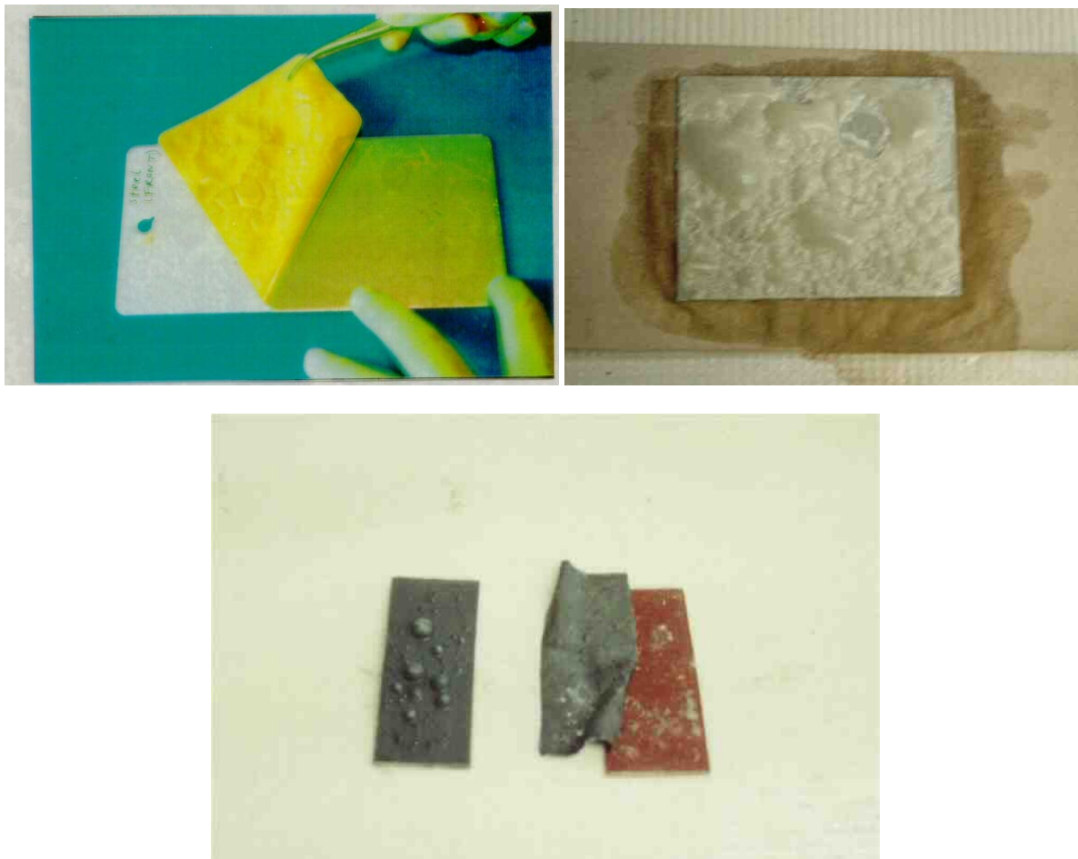
Figure 6-95: Photostripping of Paint.
