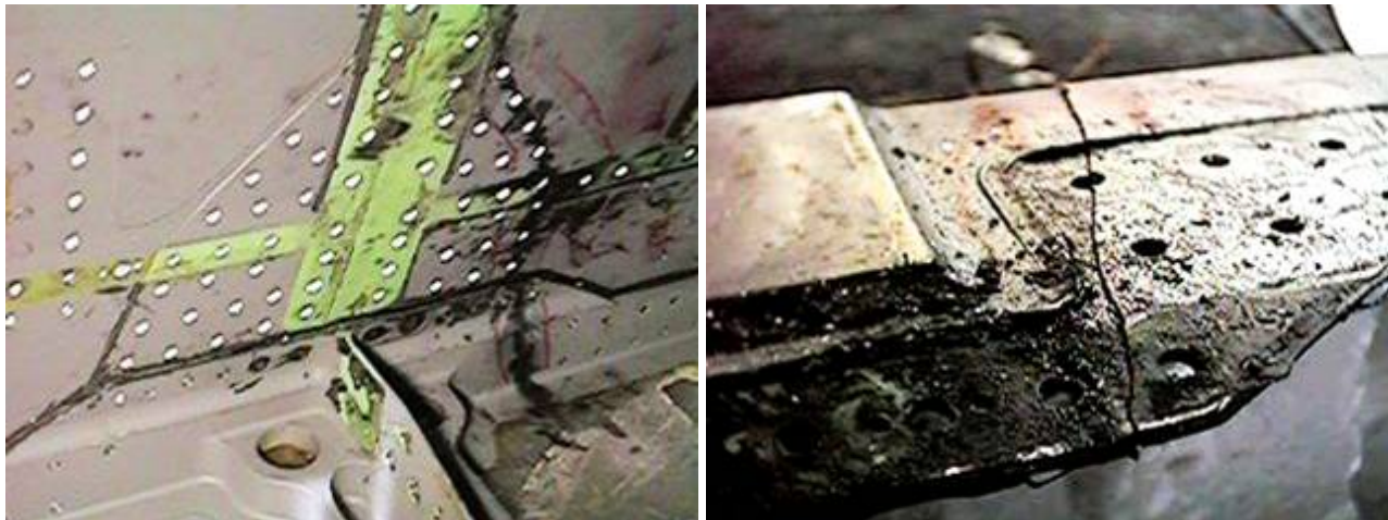
Figure 6-101: H-60 Transmission Support Beam Cracks.
