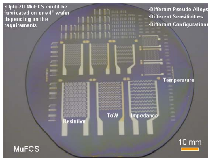
Figure 6-41: Multi-Functional Sensor (MuFCS) by BAE Systems – Different Environmental Sensors on a Single Chip.
