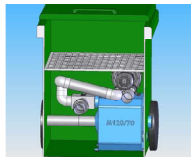
Figure 6-107: A Dehumidifier for Aircraft.
