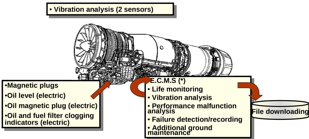
Figure 6-46: On-Board Diagnosis – Specific Sensors and Indicators in Addition to Engine Controls.
