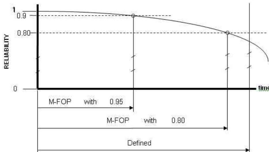
Figure 6-78: Reliability vs. Time and Probability of Maintenance-Free Operating Period (MFOP) Completion.
