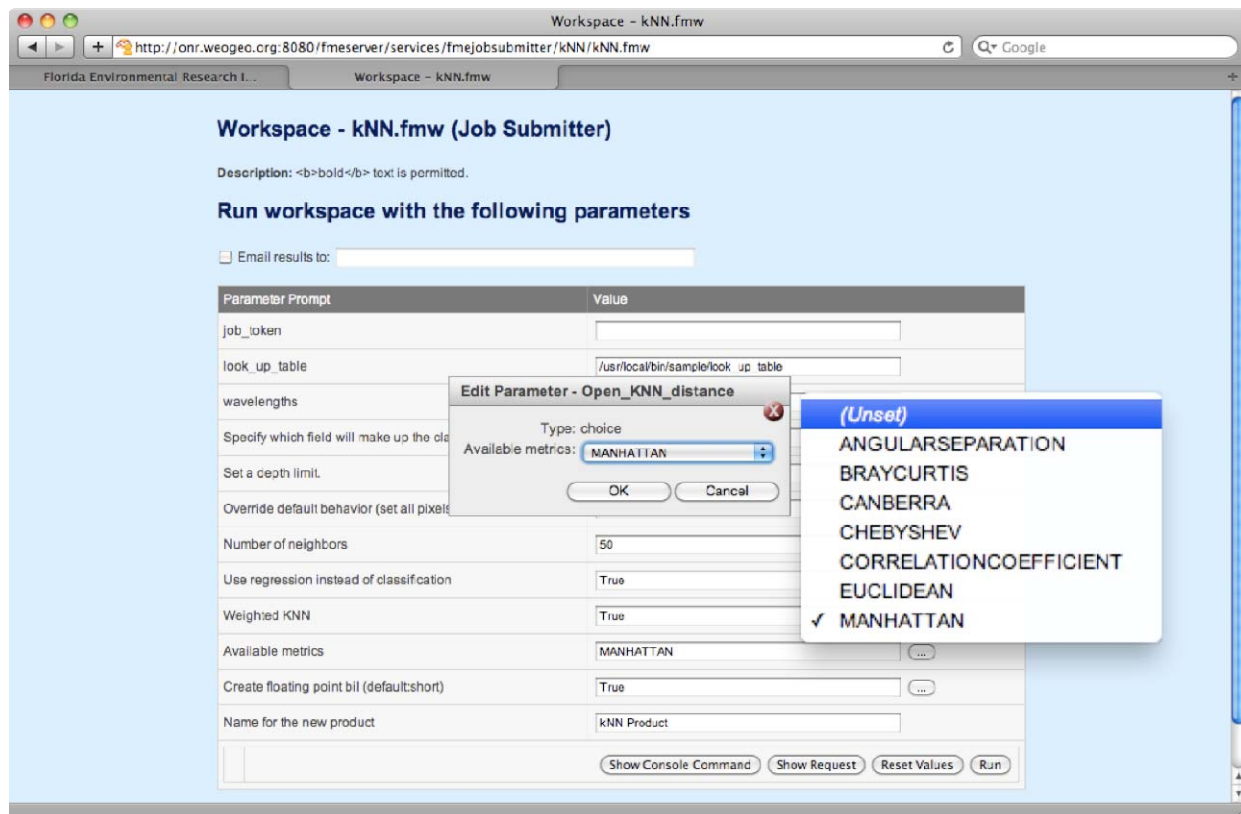
Figure 4. Parameter selection screen for the kNN algorithm on the ONR WeoGeo Library Appliance. This figure shows how drop down menus are used to select the parameters. In this example, the statistical metric to be used to match the spectrum will be Manhattan distance calculations between the database spectrum and the image spectrum.
