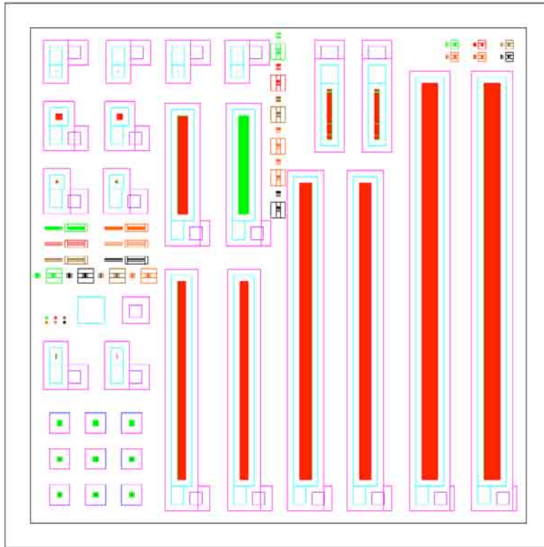
Figure 2 Die layout.
