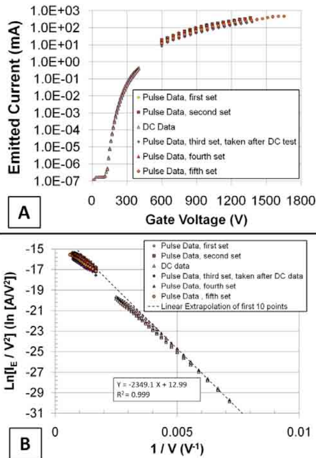
Figure 8 Characterization of a 1-million array of field emitters individually controlled by ungated FETs made of silicon with a resistivity of 34.7 \Omega \cdot \text{cm} : IV characteristics (A), FN plot of the emission current (B).
