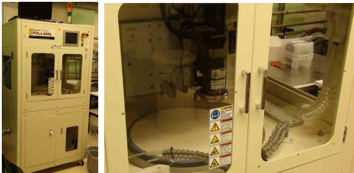
Figure 17. Front view of the installed CMP (left) and detail of the polishing pad (right).
