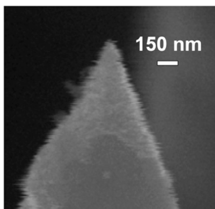
Figure 11 SEM of a typical field emitter part of of the individually ballasted FEA made of silicon with 178 \Omega\cdot\text{cm} resistivity. The tip radius is about 33 nm.
