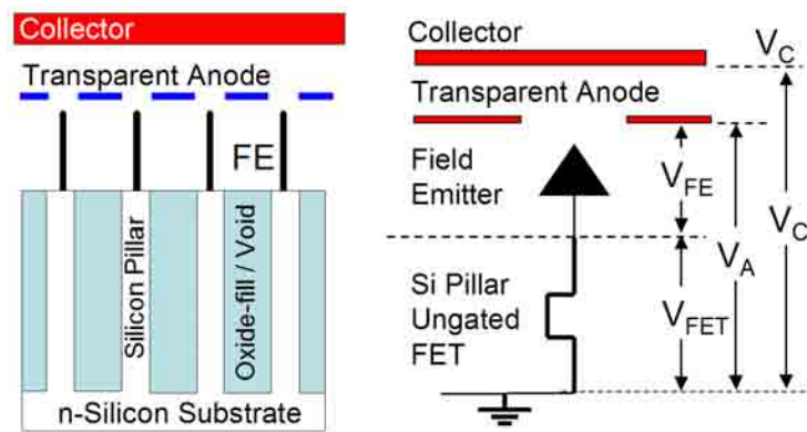
Figure 1 Device structure (left) and equivalent circuit (right). Each field emitter is fabricated on top of a different silicon column (i.e., ungated FET). The bias voltage V_A is divided between the voltage across the FE ( V_{FE} ) and the voltage across the FET ( V_{FET} ).
