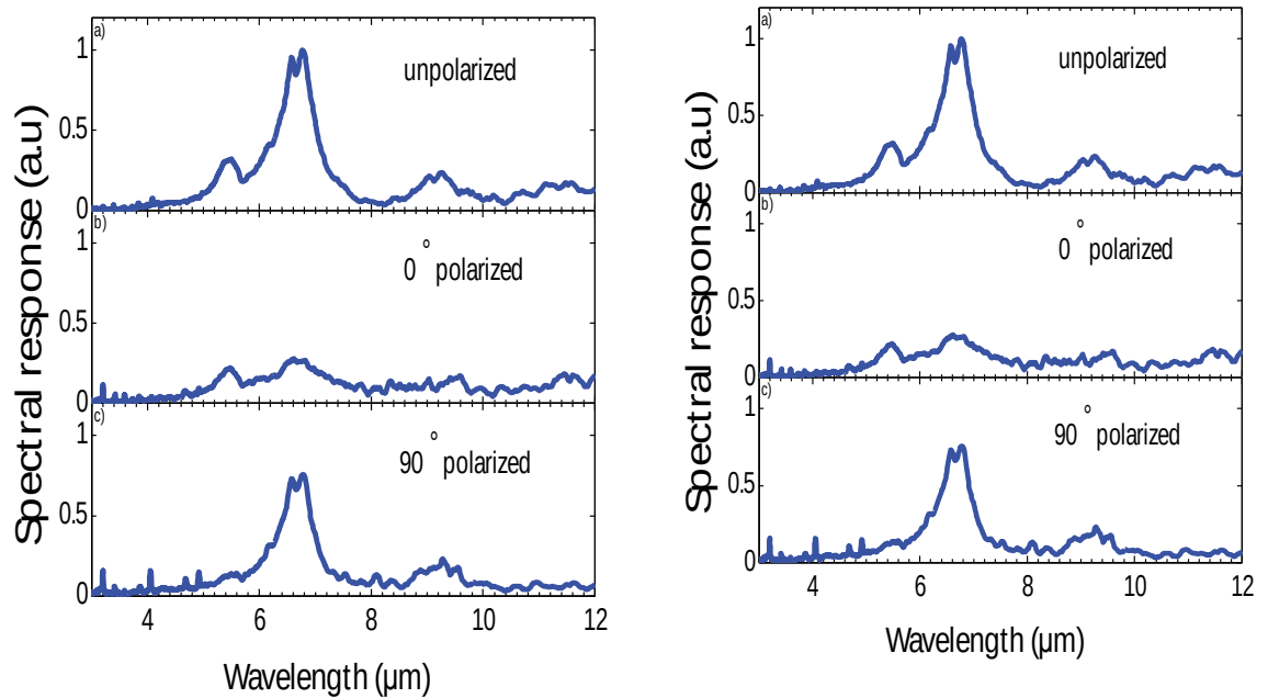
Fig.14: Polarization dependent spectral response of patterned DDWELL samples with a stretched/compressed lattice at 30 K. A peak of 6.6 \mu\text{m} is seen at 5 V bias, which is sensitive to incident polarization
