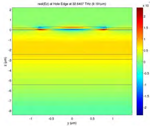
Fig 19: Y-Z mode profile of the fundamental mode of absorption in a metallic post pattern with Silver as the top metal. The mode is primarily concentrated away from the metal-semiconductor interface.
