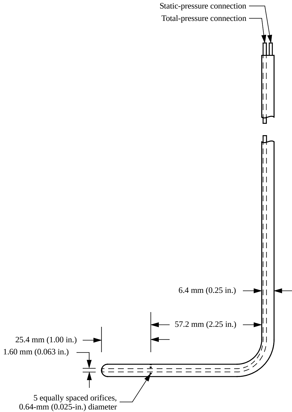
Figure 3.- Wake-survey probe.
