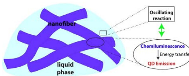
Scheme. Oscillating chemiluminescent supramolecular hydrogels
