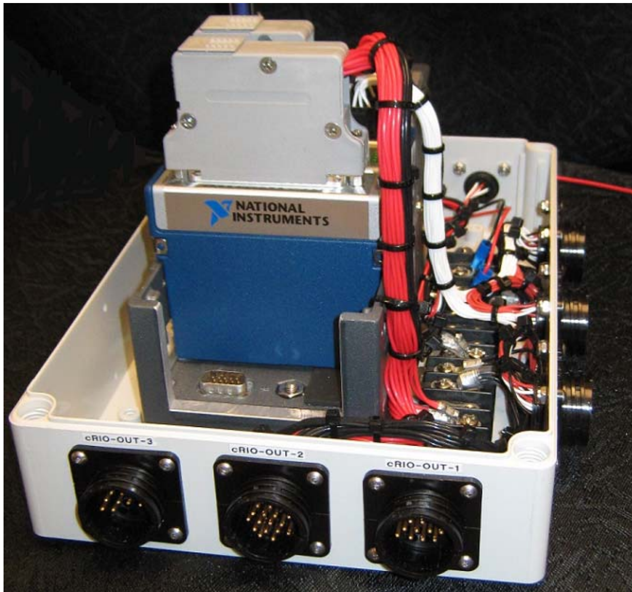
Figure 2: cRIO System with Metal Cut Out of the Chassis.
