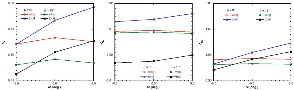
a. Lift b. Drag c. Pitch Moment Fig. 18. Lift, drag and pitch moment coefficients, vehicle trim angle = 3^\circ .
