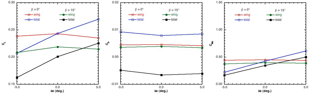
a. Lift b. Drag c. Pitch Moment Fig. 17. Lift, drag and pitch moment coefficients, vehicle trim angle = 0^\circ .
