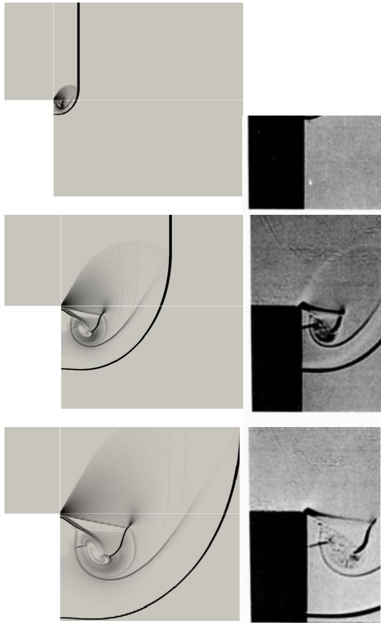
Figure 6.19: Diffraction of a Mach 2.4 shock wave down a step. Comparison between numerical schlieren and experimental images
