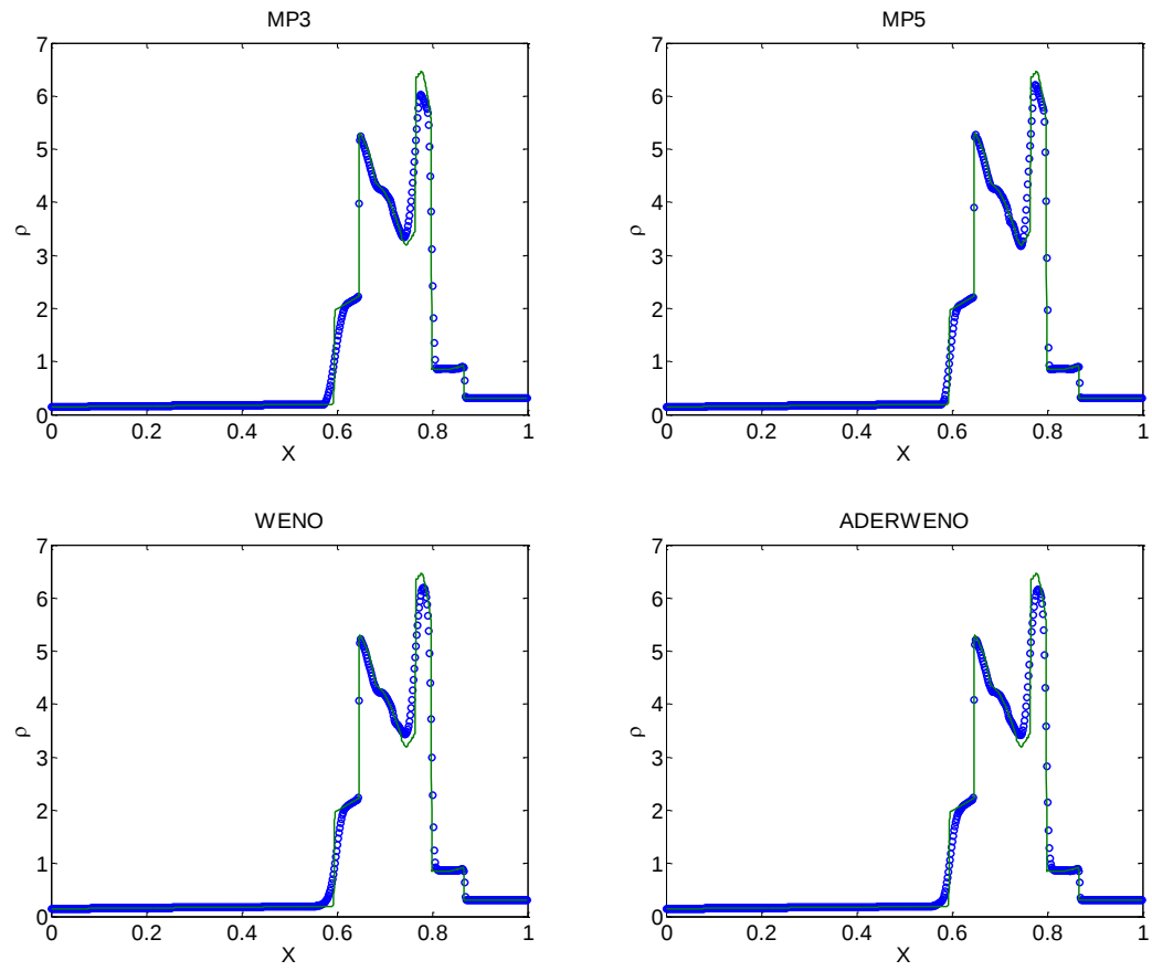
Figure 6.10: Density plot of the Blast wave problem with 600 points.
