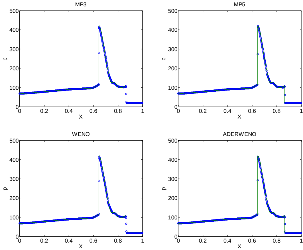
Figure 6.12: Pressure plot of the Blast wave problem with 600 points.
