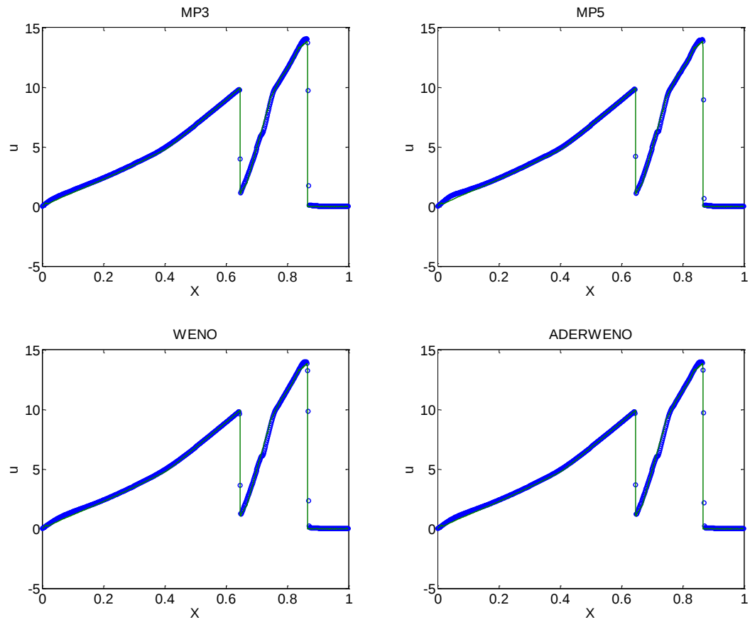
Figure 6.11: Velocity plot of the Blast wave problem with 600 points.
