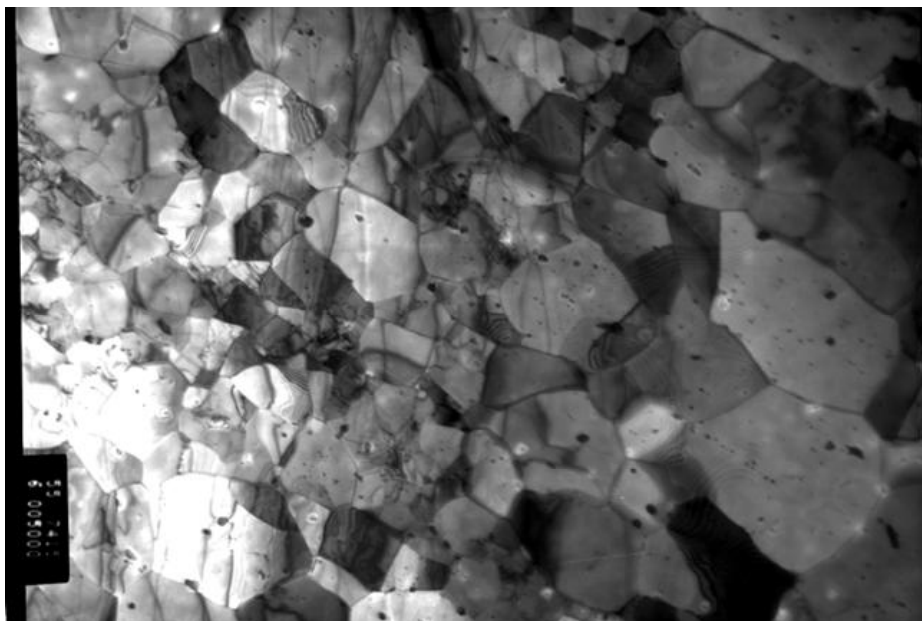
Figure 2. Bright field TEM of an Hiperco 50HS alloy subjected to an anneal of 700°C for 4hr. Average grain size of about 0.7μm.
