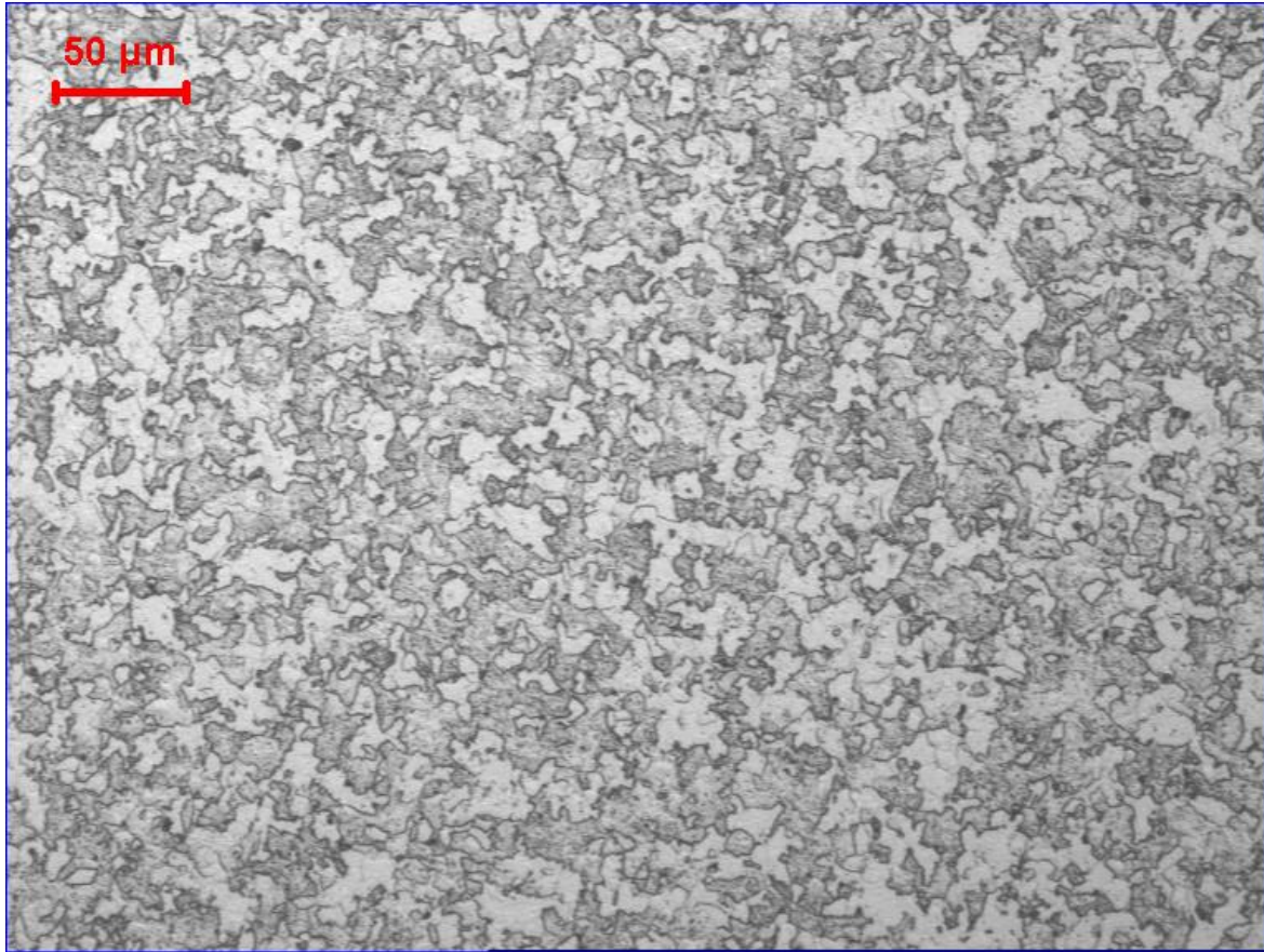
Figure 4. Optical micrograph of an Hiperco 50HS alloy subjected to an anneal of 1000°C for 1hr. Average grain size of about 16μm.
