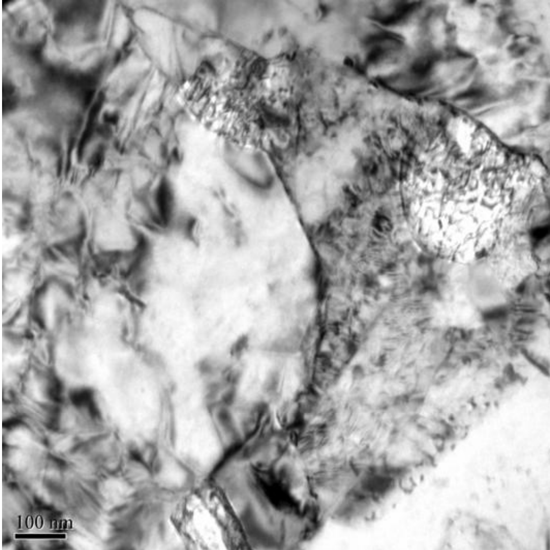
Figure 7. Bright field TEM of Hiperco 50HS alloy subjected to an anneal of 1200°C for 1hr. Average grain size of about 161 \mu m. A subgrain structure is displayed.
