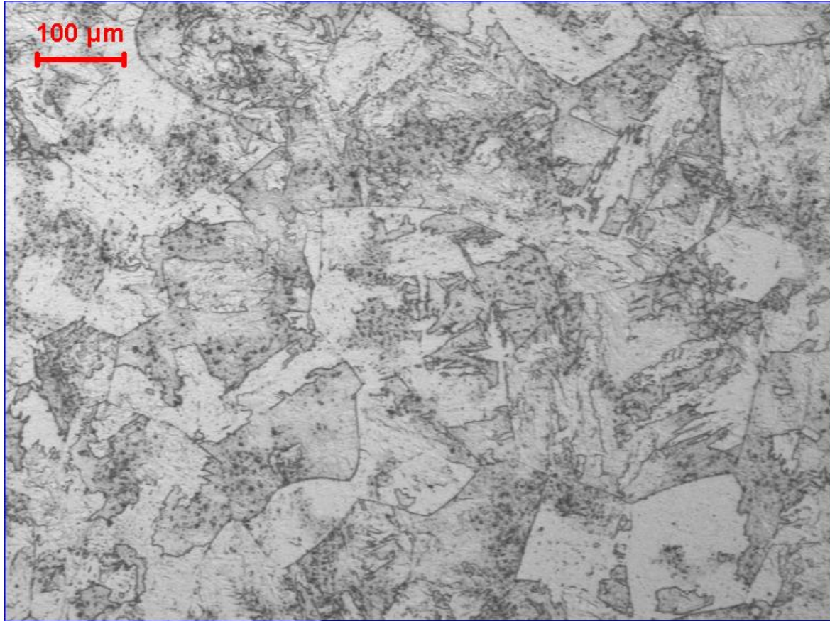
Figure 5. Optical micrograph of an Hiperco 50HS alloy subjected to an anneal of 1100°C for 1hr. Average grain size of about 70μm.
