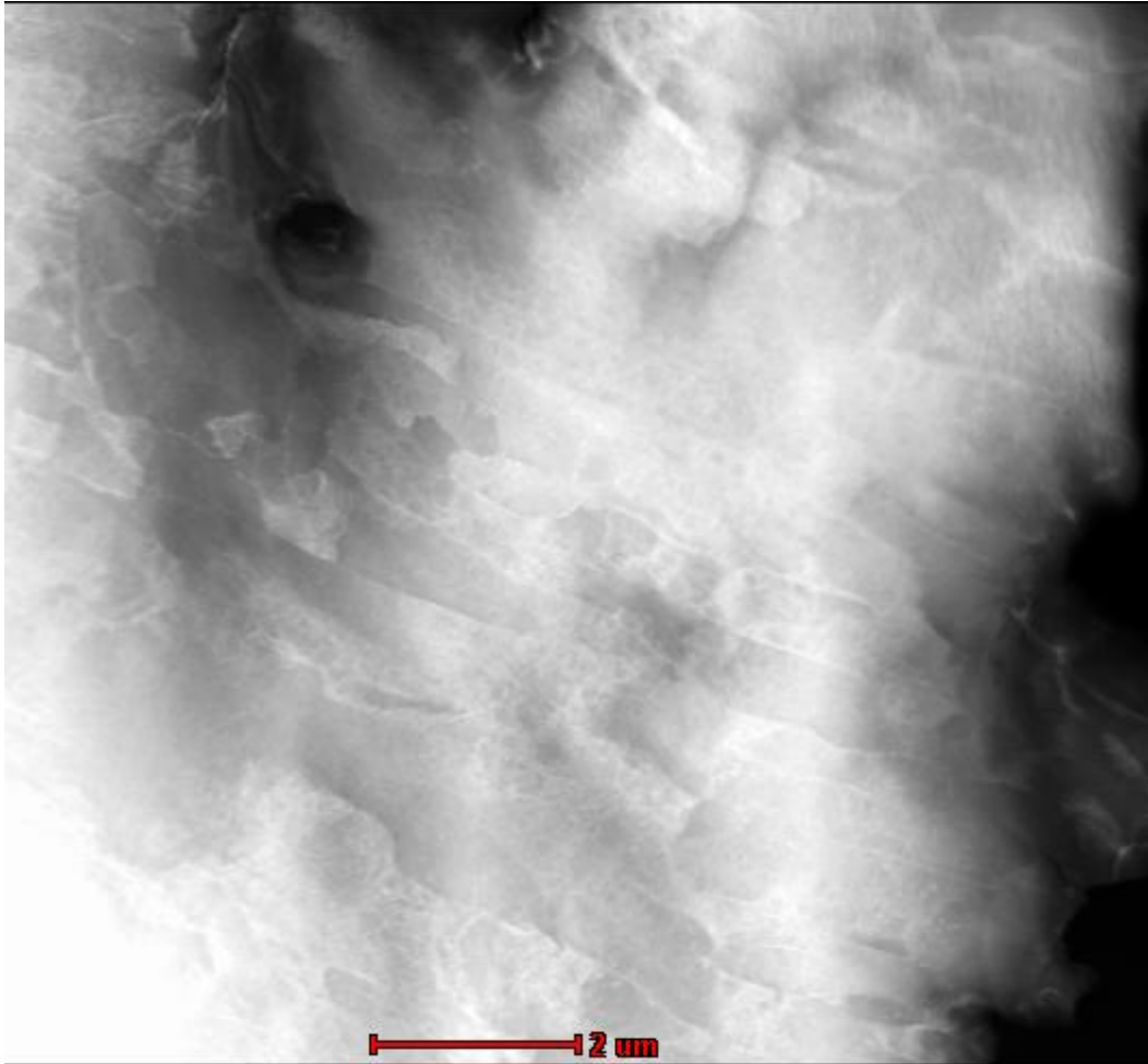
Figure 8. Higher magnification dark field TEM of an Hiperco 50HS alloy subjected to an anneal of 1200°C for 1hr displaying subgrain of size about 1μm.
