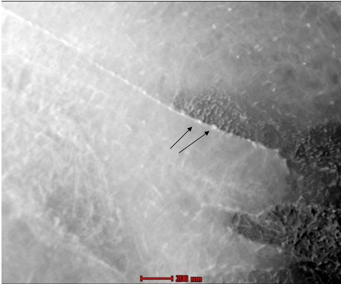
Figure 9. Bright field TEM of Hiperco 50HS alloy subjected to an anneal of 1200°C for 1hr. Arrows point to apparent precipitates at the subgrain boundaries.
