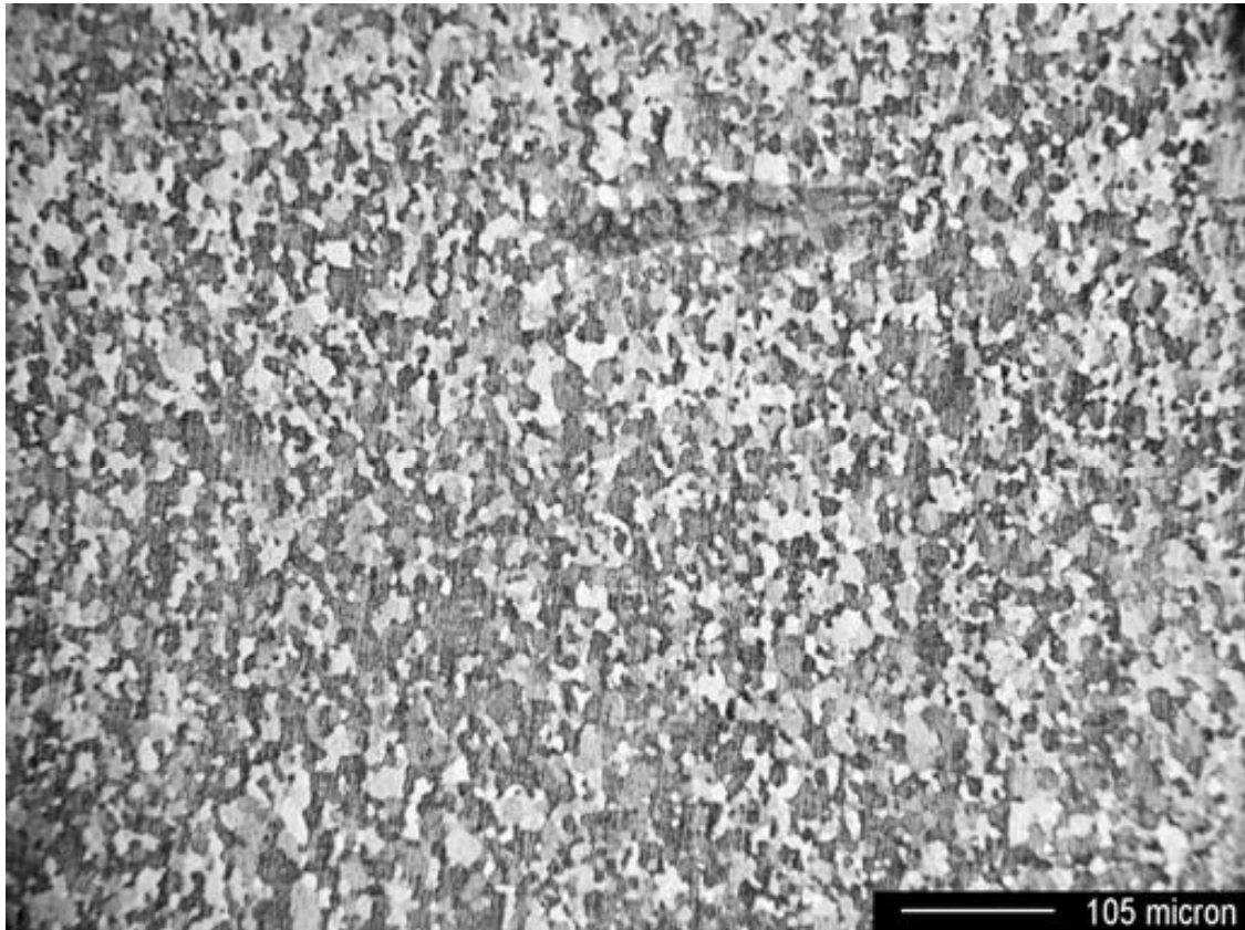
Figure 3. Optical micrograph of an Hiperco 50HS alloy subjected to an anneal of 843°C for 2hr. Average grain size of about 10 \mu m.
