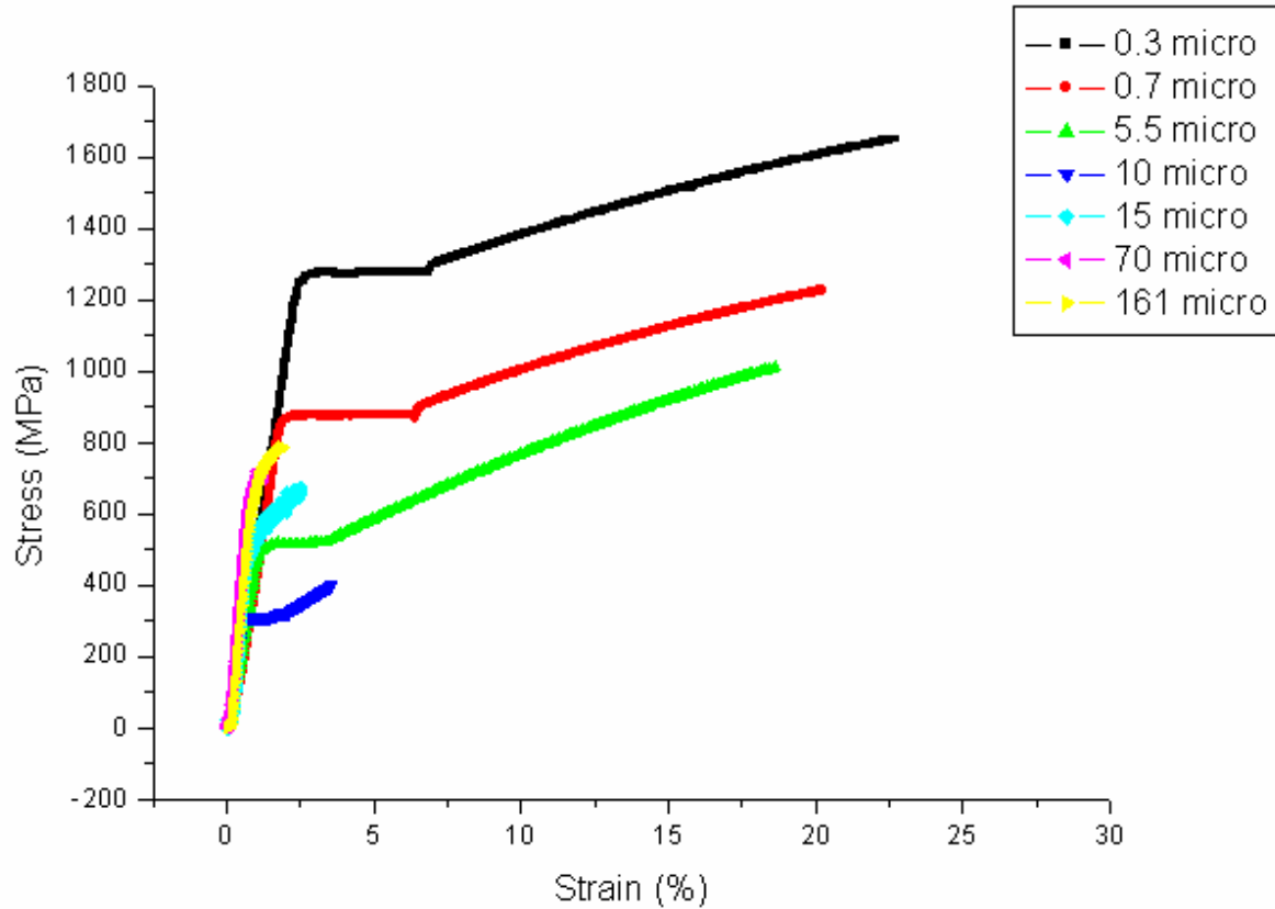
Figure 10. Room temperature tensile stress-strain curves for annealed 50HS alloys with different grain sizes.
