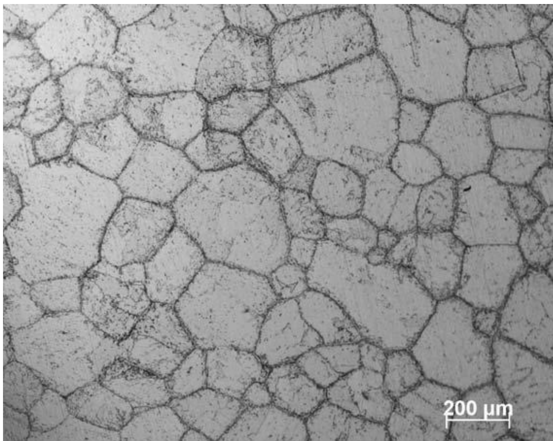
Figure 6. Optical micrograph of Hiperco 50HS alloy subjected to an anneal of 1200°C for 1hr. Average grain size of about 161μm.
