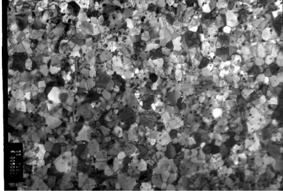
Figure 1. Bright field TEM of an Hiperco 50HS alloy subjected to an anneal of 650°C for 4hr. Average grain size of about 0.3μm.
