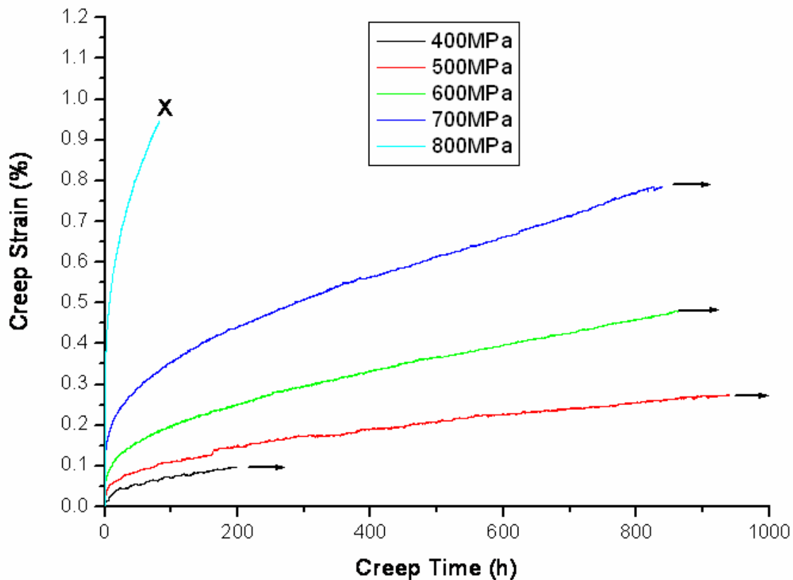
Figure 11. Creep strain for different applied stresses at 500°C as a function of time for Hiperco 50HS with average grain size of 161 \mu m.
