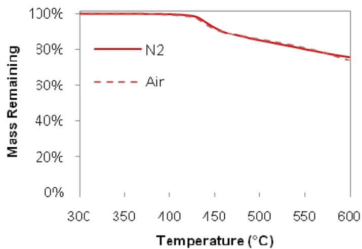
Figure 9: TGA of (a) monomer 9 and (b) PT-30 under nitrogen and air
