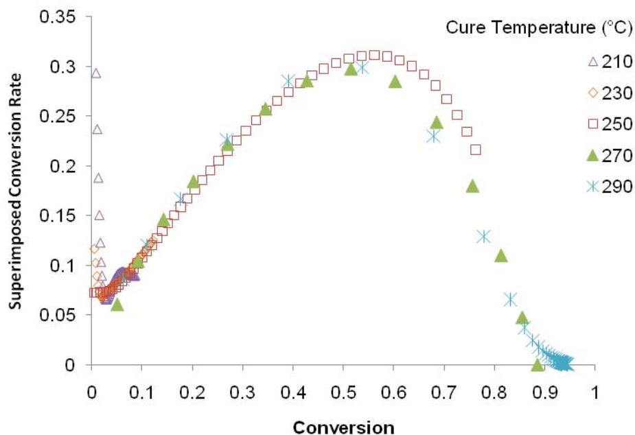
Figure S-5. Superimposed conversion rate curves for (a) monomer 9 and (b) PT-30; the superposition factors are for (a) Scaling: 0.006, 0.012, 0.034, 0.095, 0.2; Offset: -0.0026, 0.001, -0, 0.003, 0 (b) Scaling: 0.01, 0.05, 0.16, 0.42, 1; Offset: 0.0022, 0, 0, 0.005, 0, in ascending order of temperature, where the original rate (/min.) = displayed rate * scaling + offset.
