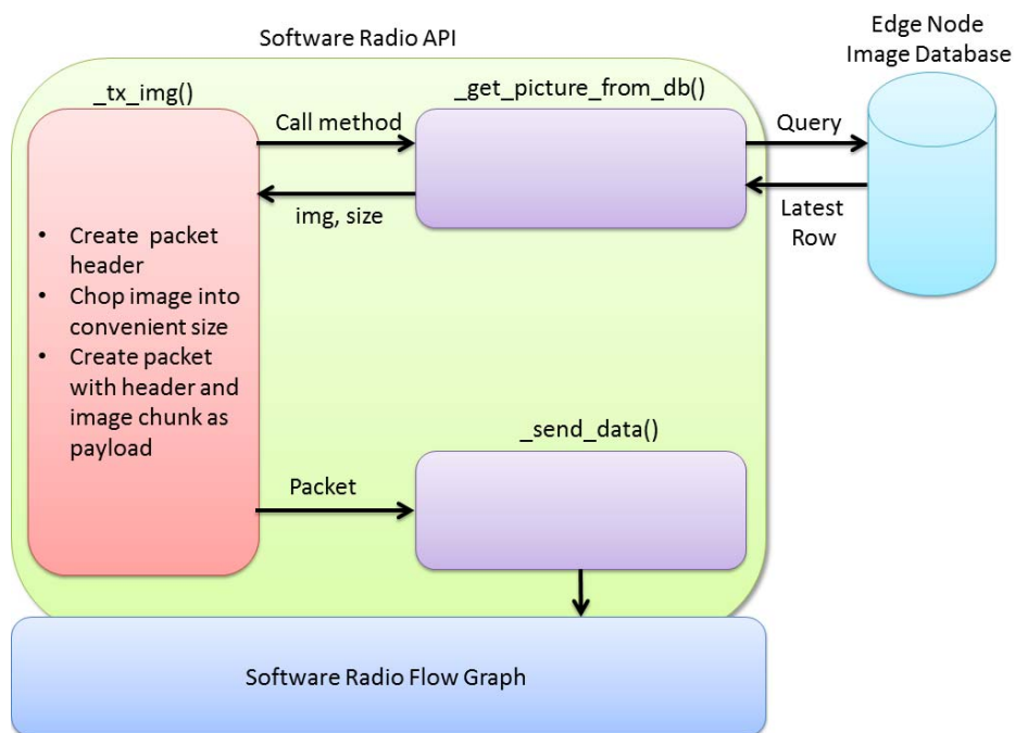
Figure 11 Preparing image frames for transport over RF downlink.
