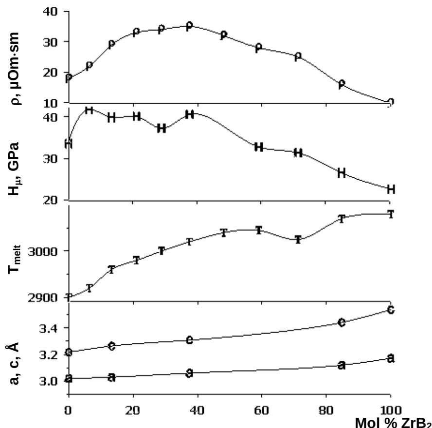
Fig. 11. – Concentration dependences of lattice parameters, (“a” and “c”), specific resistance ( \rho ), microhardness (H) and melting points (T) for (Ti, Zr)B 2 solid solutions [16].
