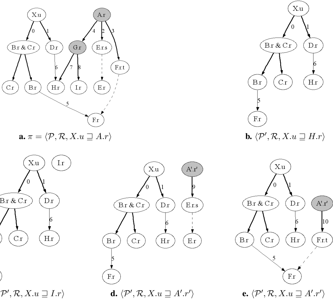
Figure 5: Decomposition example 2
