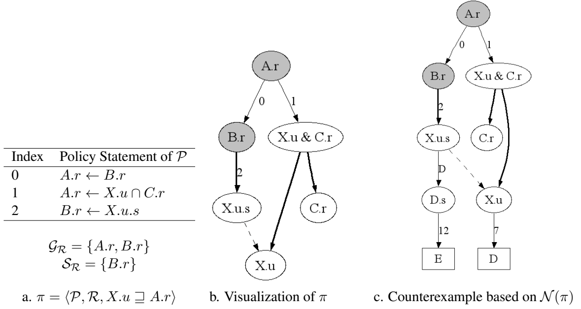
Figure 6: Running example
