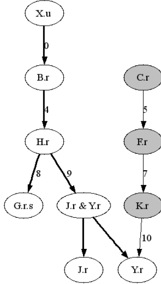
c. \pi_2
