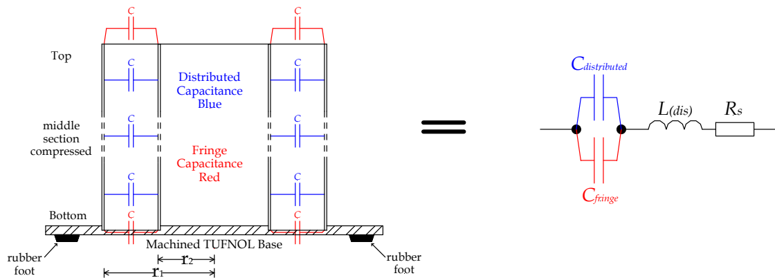
Figure 4: Cross-sectional view of the co-axial test cell mounted on a machined TUFNOL base showing the distributed capacitances and the cell's equivalent electrical circuit
