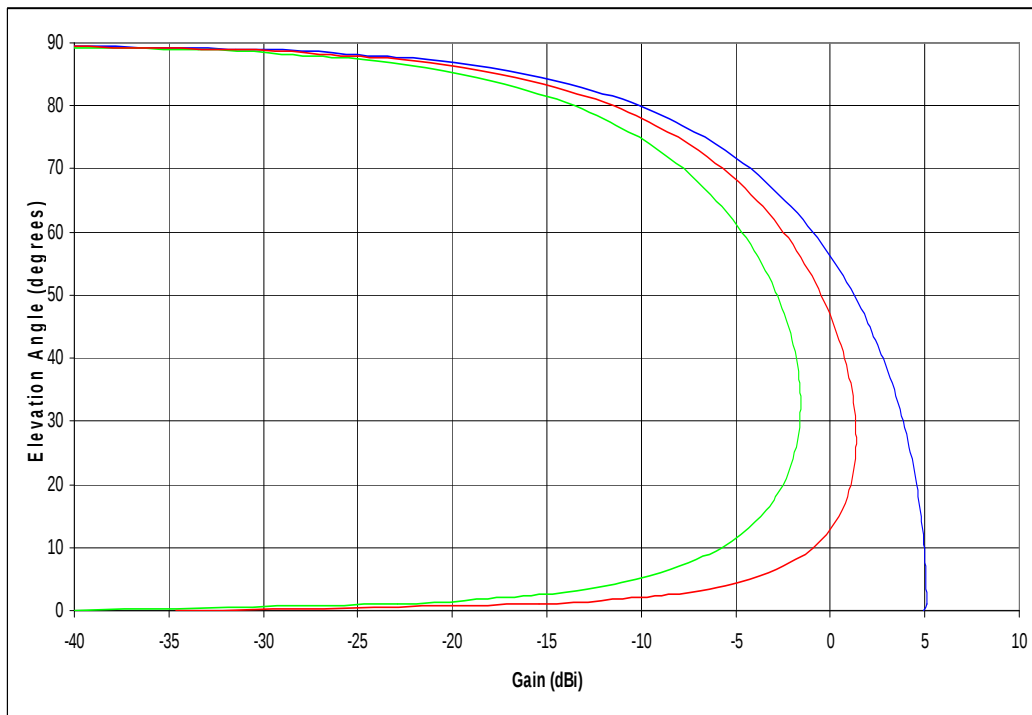
Figure C1: Simulated gain in dBi of the 6.5 m resonant monopole at 11.27 MHz using the above equations (C1) and (C2)
