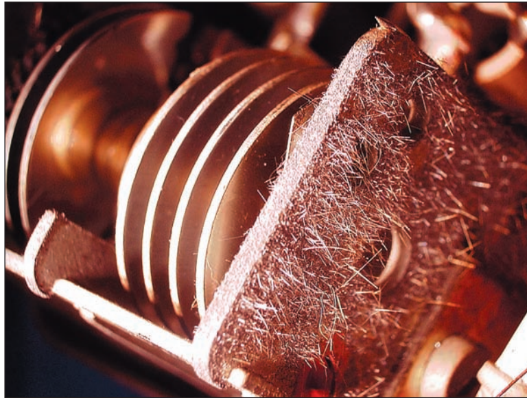
Figure 6: Example of a Capacitor with Tin Whiskers
