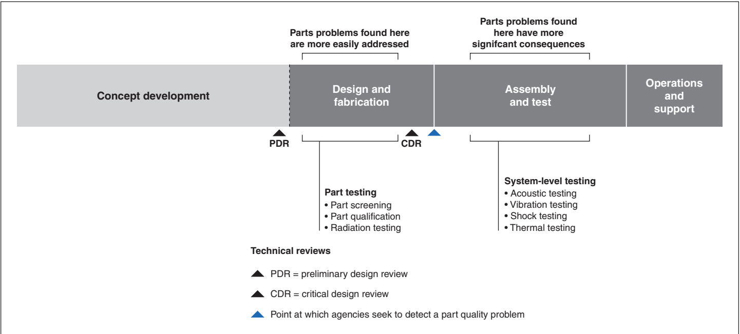
Figure 5: Summary of Typical Key Testing Practices to Identify Parts Quality Problems
