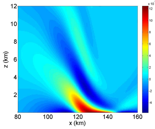
(a) u (m/s) t = 1200 s
