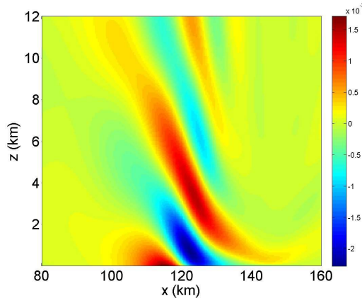
(e) w (m/s) t = 1200 s
