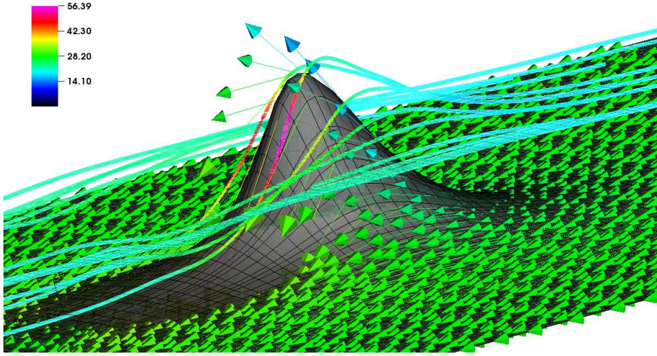
Figure 8: Streamlines and velocity vectors produced by flow about a nonlinear mountain with h = 1000 m.
