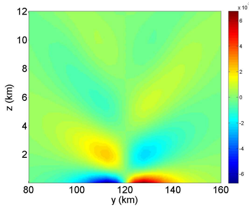
(c) v (m/s) t = 1200 s
