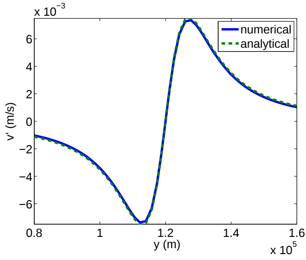
(b) cross-stream velocity
