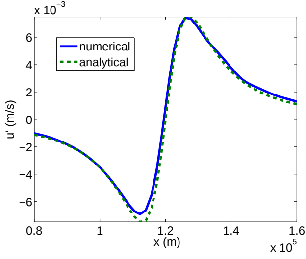
(a) down-stream velocity
