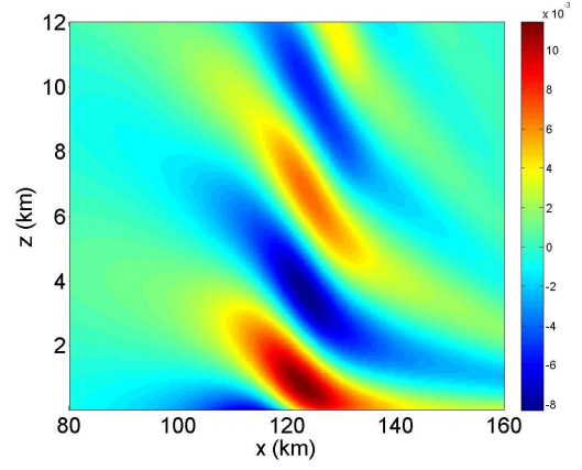
(b) u (m/s) t = 3600 s
