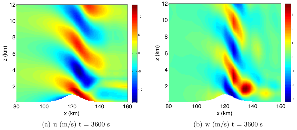
Figure 9: Horizontal and vertical velocities in the plane y = 0 for flow over a nonlinear mountain with h = 1000 m.
