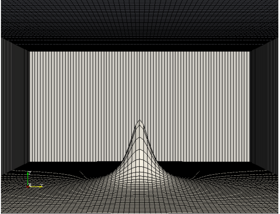
Figure 3: Profile of the isolated, 3D linear hydrostatic mountain defined by Eq. (27) originally considered in [33]
