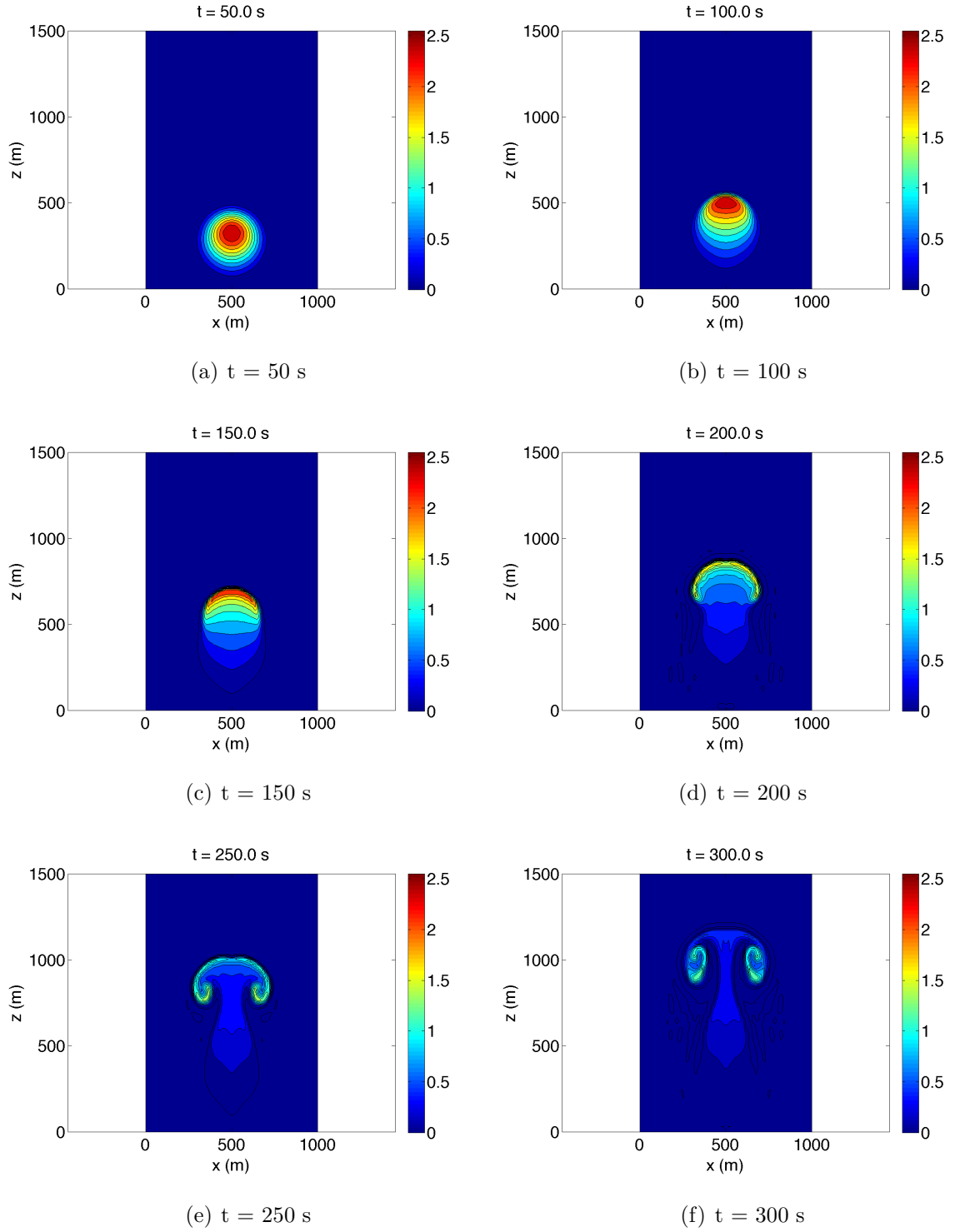
Figure 10: Evolution of a 3D rising thermal bubble problem ( x-z -slices of the potential temperature perturbation \theta' ) in the y = 500 m plane for t = 50, 100, 150, 200, 250 , and 300 seconds.
