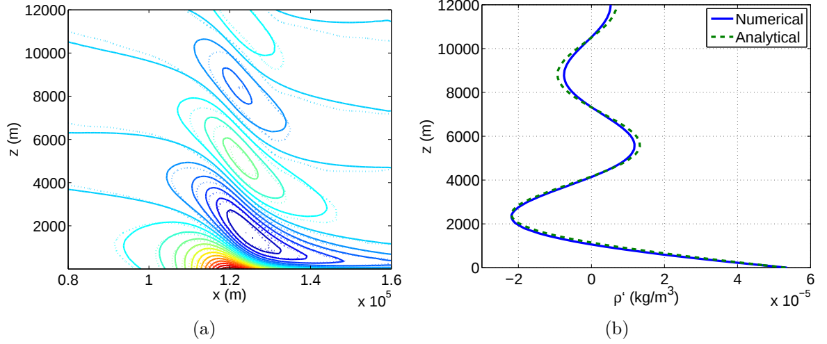
Figure 6: Comparison of the density perturbations \rho' for the isolated linear hydrostatic mountain using 1) NUMA and 2) a contour integral solution [34]. In panel a), the \rho' contours in the plane y = 0 are shown. In panel b), \rho' is shown as a function of z using x = y = 0 .
