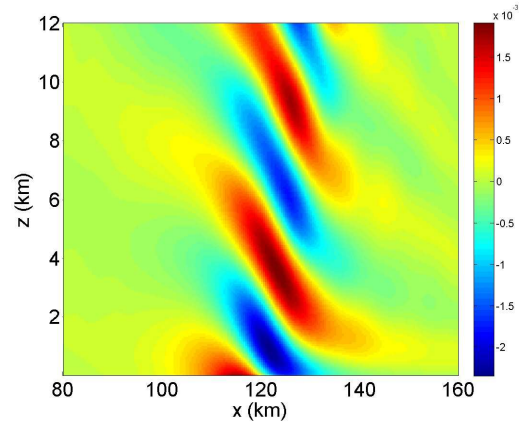
(f) w (m/s) t = 3600 s
