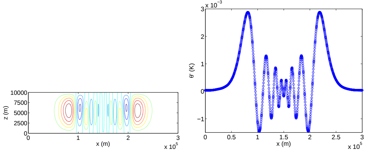
Figure 4: Case 1: 2D Inertia-gravity waves. Potential temperature perturbation after 2500 s for 250 m resolution (120 by 1 by 4 elements) and 10-th order polynomials. a) shows a slice in the center of the domain and b) shows profiles along z = 5000 m.
