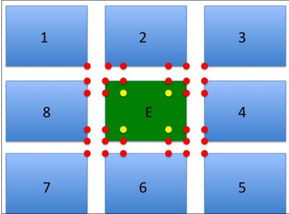
Figure 2: Global DSS operator in a 2D setting, where each processor owns one element. The element E (green) requires nodal information for its 8 nodal neighbors in order to construct the RHS operator on the boundary (red dots). However, the interior nodes (yellow dots) do not need to be communicated to adjacent processors, resulting in a halo-free algorithm.
