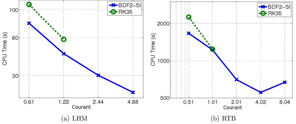
Figure 11: Comparison of the explicit RK35 and semi-implicit BDF2 time-integrators in serial mode for a) the linear hydrostatic mountain problem and 2) the 3D rising thermal bubble problem. In both cases and for all applicable Courant numbers, the BDF2-SI integrator is more efficient.
