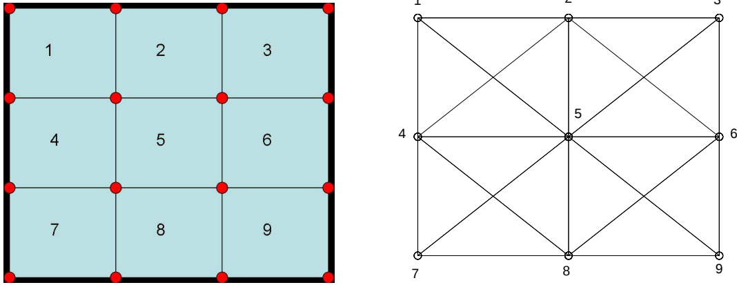
Figure 1: Example 2D grid (left) and the associated adjacency graph. Since spectral element methods utilize nodal communication, the adjacency graph includes both edge and vertex connectivity, with a maximum degree of eight. For 3D, structured, Cartesian grids, the maximum degree is 26.
