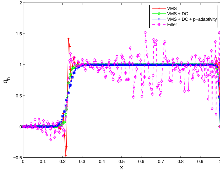
Figure 10: St\text{-}2D : steady-state solution on 50 \times 50 4^{th} -order elements. Vertical slice at z = 0.3
